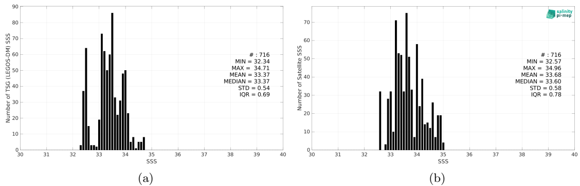
Figure 2: Histograms of SSS from TSG (LEGOS-DM) (a) and SMAP SSS L2 v5.0 (JPL) (b) considering all match-up pairs per bins of 0.1 over the Bay of Bengal Pi-MEP region and for the full satellite product period.
