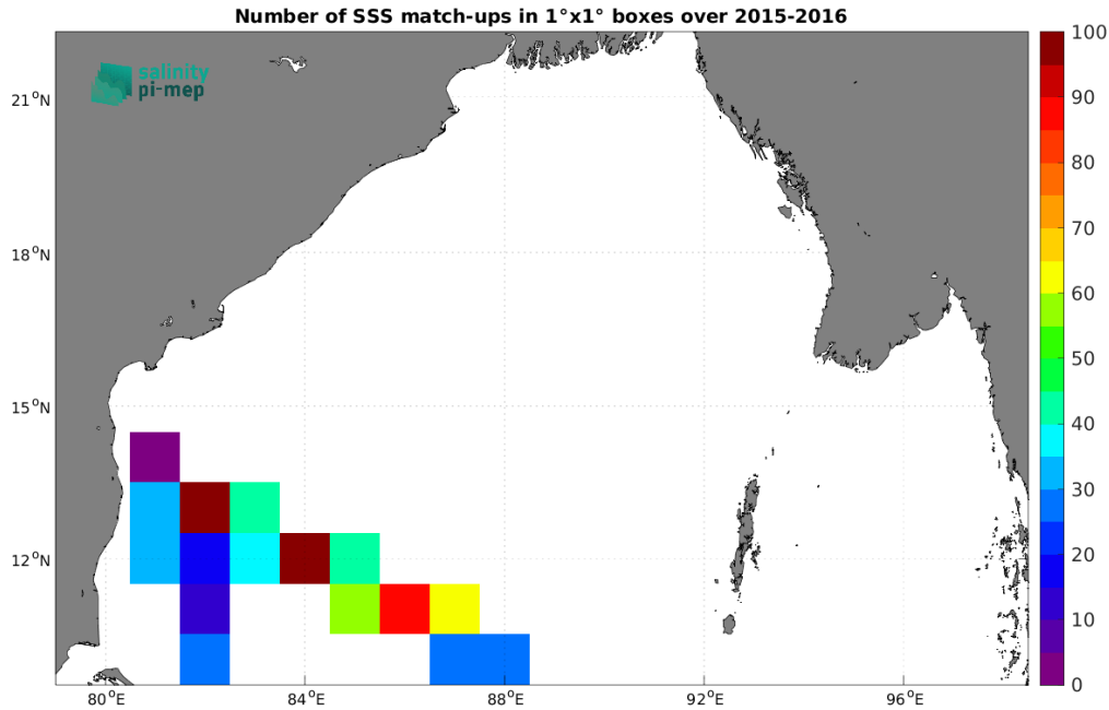
Figure 4: Number of SSS match-ups between TSG (LEGOS-DM) SSS and the SMAP SSS L2 v5.0 (JPL) SSS product for the Bay of Bengal Pi-MEP region over 1^\circ \times 1^\circ boxes and for the full satellite product period.
