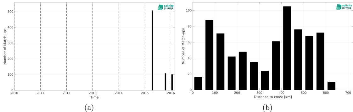
Figure 1: Number of match-ups between TSG (LEGOS-DM) and SMAP SSS L2 v5.0 (JPL) SSS as a function of time (a) and as function of the distance to coast (b) over the Bay of Bengal Pi-MEP region and for the full satellite product period.
