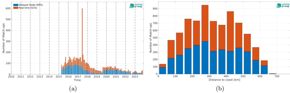
Figure 1: Number of match-ups between Argo and SMAP SSS L2 v5.0 (JPL) SSS as a function of time (a) and as function of the distance to coast (b) over the Bay of Bengal Pi-MEP region and for the full satellite product period.
