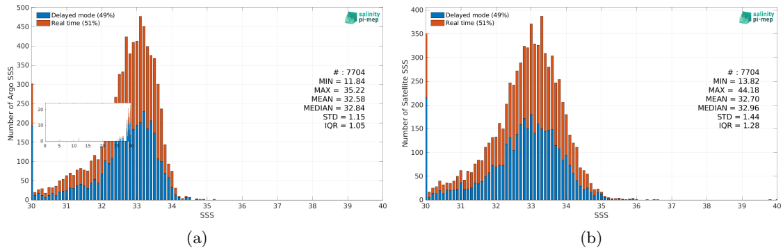
Figure 2: Histograms of SSS from Argo (a) and SMAP SSS L2 v5.0 (JPL) (b) considering all match-up pairs per bins of 0.1 over the Bay of Bengal Pi-MEP region and for the full satellite product period.
