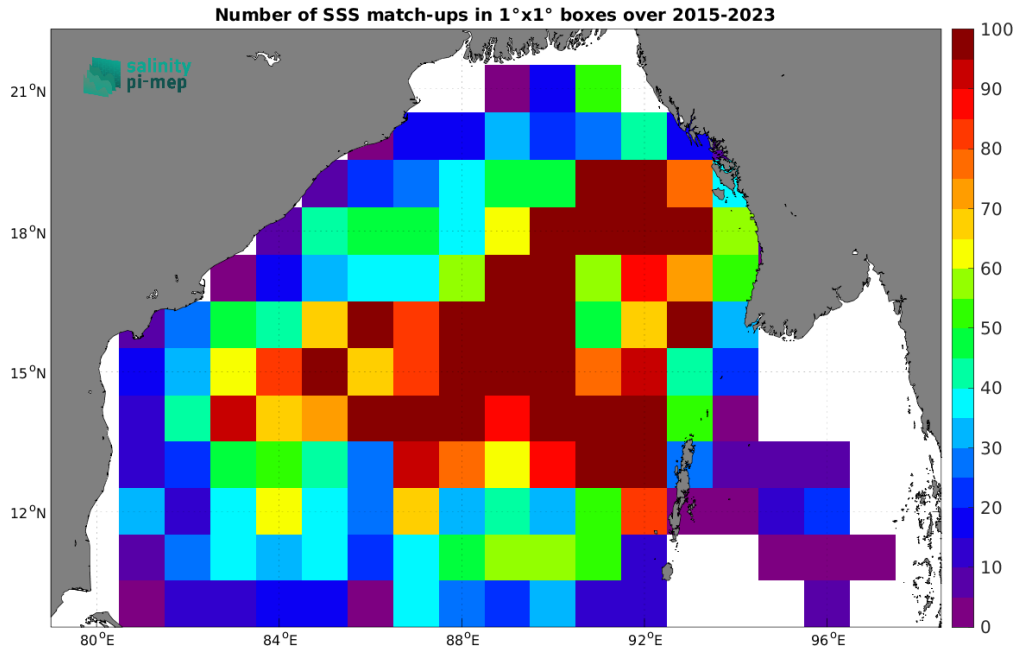
Figure 4: Number of SSS match-ups between Argo SSS and the SMAP SSS L2 v5.0 (JPL) SSS product for the Bay of Bengal Pi-MEP region over 1^\circ \times 1^\circ boxes and for the full satellite product period.
