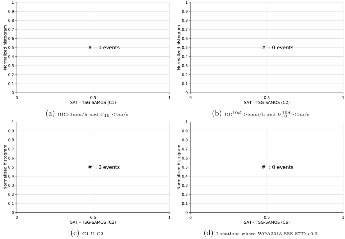
Figure 13: Normalized histogram of \Delta SSS (SMAP-L2-JPL-V4 - TSG-SAMOS) for 6 different subdatasets corresponding to: RR > 1\text{mm/h} and U_{10} < 5\text{m/s} (a), RR^{10d} > 5\text{mm/h} and U_{10}^{10d} < 5\text{m/s} (b), C1 \cup C2 (c), Locations where WOA2013 SSS STD > 0.2 (d).
