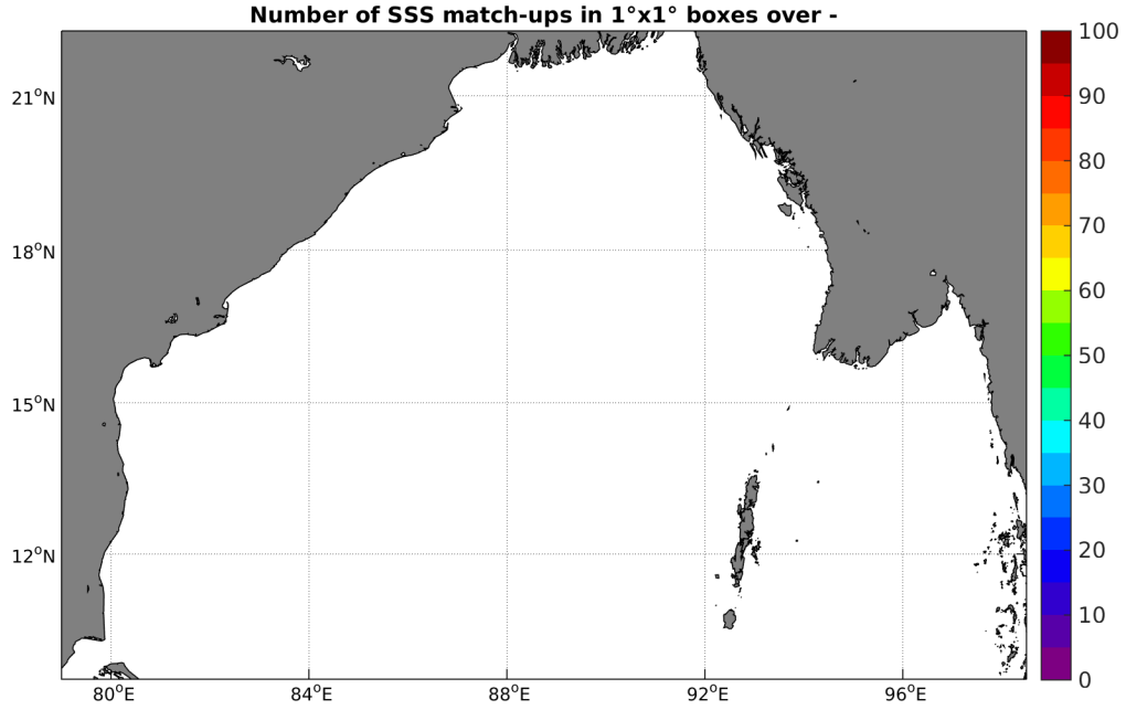
Figure 4: Number of SSS match-ups between TSG-SAMOS SSS and the SMAP-L2-JPL-V4 SSS product for the Bay of Bengal Pi-MEP region over 1^\circ \times 1^\circ boxes and for the full satellite product period.
