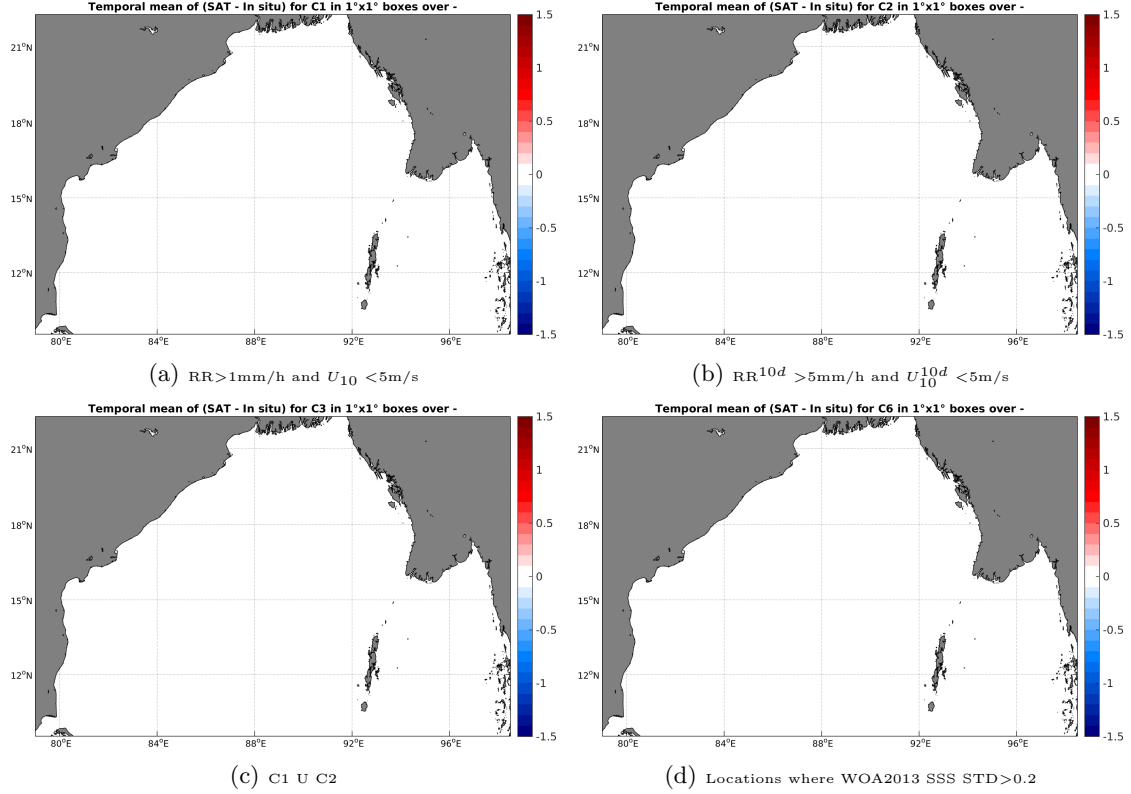
Figure 12: Temporal mean gridded over spatial boxes of size 1^\circ \times 1^\circ of \Delta SSS (SMAP-L2-JPL-V4 - TSG-SAMOS) for 4 different subdatasets corresponding to: RR > 1 mm/h and U_{10} < 5 m/s (a), RR 10d > 5 mm/h and U_{10}^{10d} < 5 m/s (b), C1 U C2 (c), Locations where WOA2013 SSS STD > 0.2 (d).
