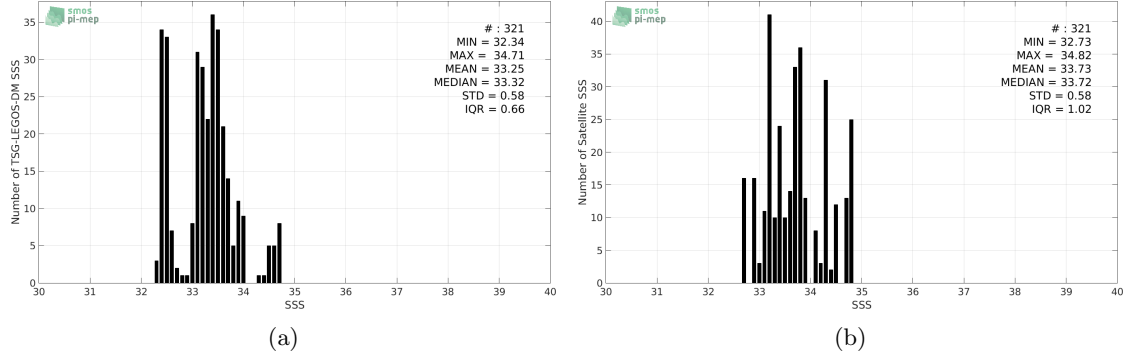
Figure 2: Histograms of SSS from TSG-LEGOS-DM (a) and SMAP-L2-JPL-V4 (b) considering all match-up pairs per bins of 0.1 over the Bay of Bengal Pi-MEP region and for the full satellite product period.
