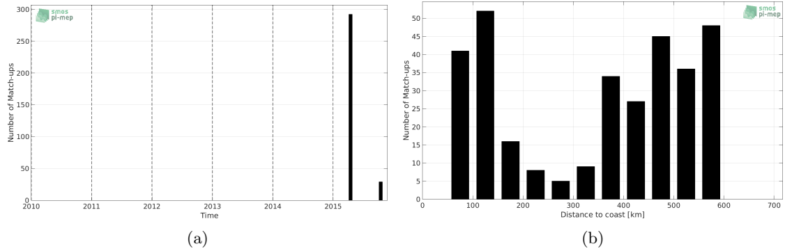
Figure 1: Number of match-ups between TSG-LEGOS-DM and SMAP-L2-JPL-V4 SSS as a function of time (a) and as function of the distance to coast (b) over the Bay of Bengal Pi-MEP region and for the full satellite product period.
