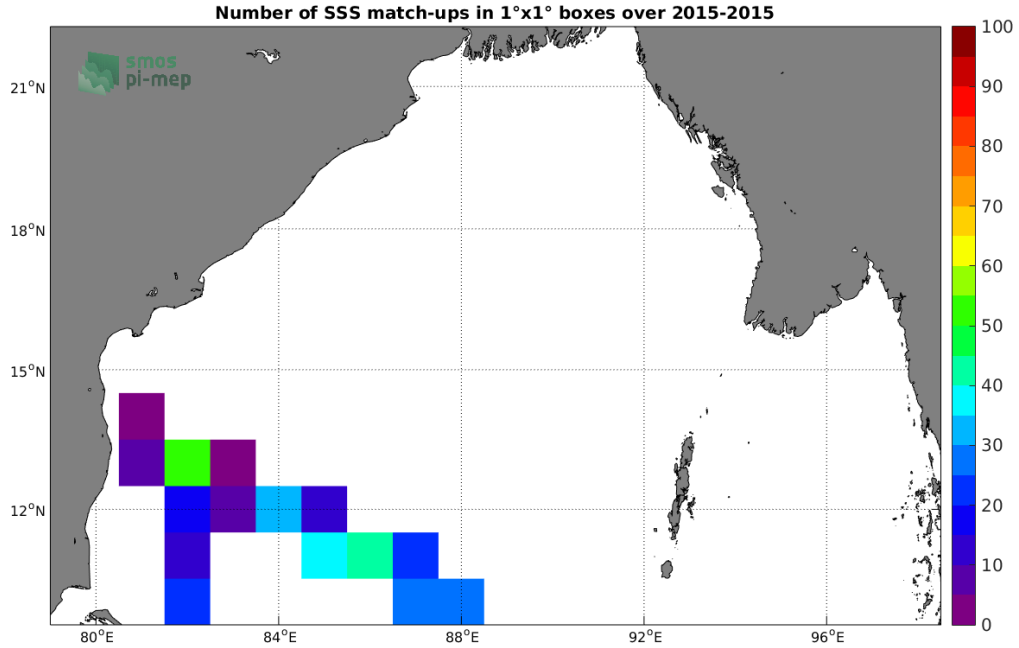
Figure 4: Number of SSS match-ups between TSG-LEGOS-DM SSS and the SMAP-L2-JPL-V4 SSS product for the Bay of Bengal Pi-MEP region over 1°x1° boxes and for the full satellite product period.
