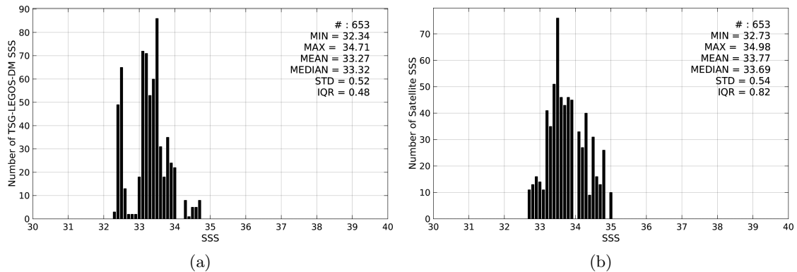
Figure 2: Histograms of SSS from TSG-LEGOS-DM (a) and SMAP-L2-JPL-V4 (b) considering all match-up pairs per bins of 0.1 over the Bay of Bengal Pi-MEP region and for the full satellite product period.
