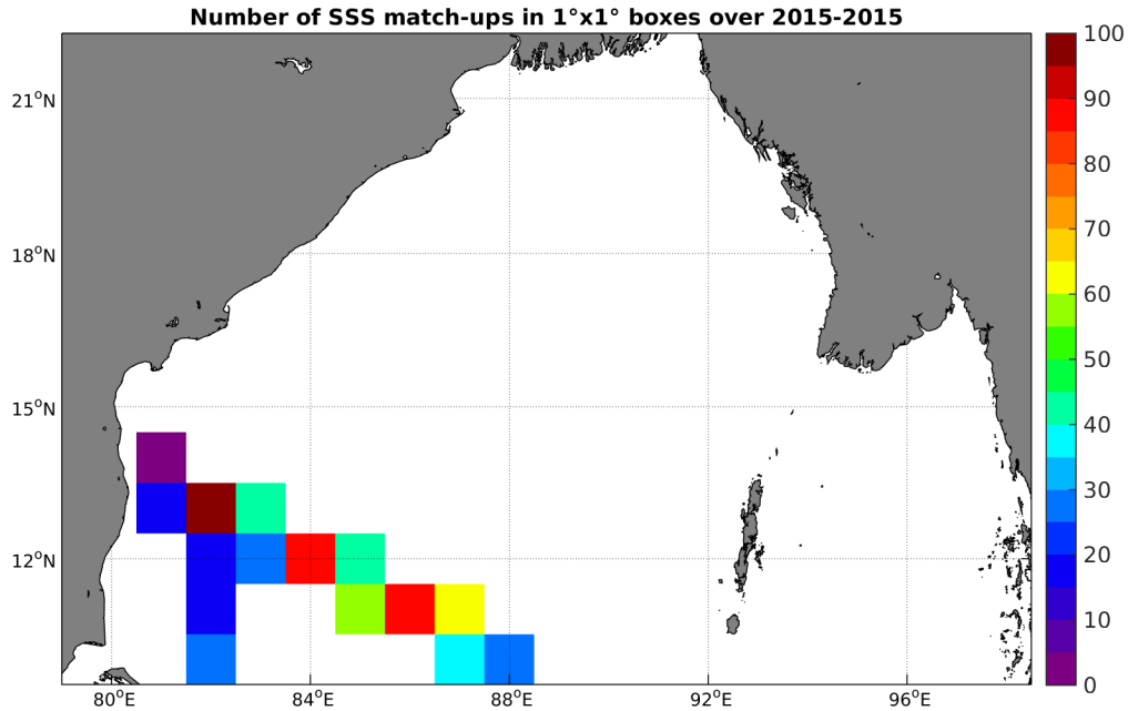
Figure 4: Number of SSS match-ups between TSG-LEGOS-DM SSS and the SMAP-L2-JPL-V4 SSS product for the Bay of Bengal Pi-MEP region over 1^\circ \times 1^\circ boxes and for the full satellite product period.
