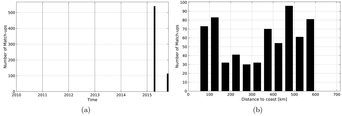
Figure 1: Number of match-ups between TSG-LEGOS-DM and SMAP-L2-JPL-V4 SSS as a function of time (a) and as function of the distance to coast (b) over the Bay of Bengal Pi-MEP region and for the full satellite product period.
