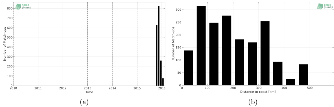
Figure 1: Number of match-ups between Surface drifters and SMAP-L2-JPL-V4 SSS as a function of time (a) and as function of the distance to coast (b) over the Bay of Bengal Pi-MEP region and for the full satellite product period.
