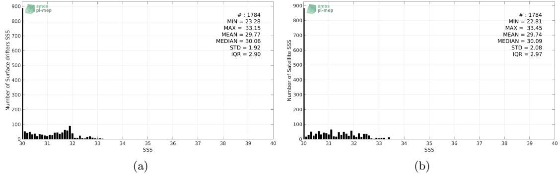
Figure 2: Histograms of SSS from Surface drifters (a) and SMAP-L2-JPL-V4 (b) considering all match-up pairs per bins of 0.1 over the Bay of Bengal Pi-MEP region and for the full satellite product period.
