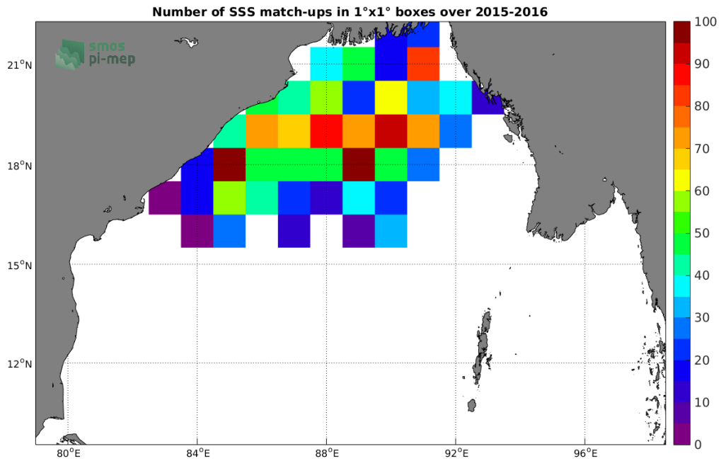
Figure 3: Number of SSS match-ups between Surface drifters SSS and the SMAP-L2-JPL-V4 SSS product for the Bay of Bengal Pi-MEP region over 1°x1° boxes and for the full satellite product period.
