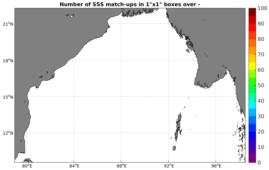
Figure 3: Number of SSS match-ups between Surface drifters SSS and the SMAP-L2-JPL-V4 SSS product for the Bay of Bengal Pi-MEP region over 1^\circ \times 1^\circ boxes and for the full satellite product period.
