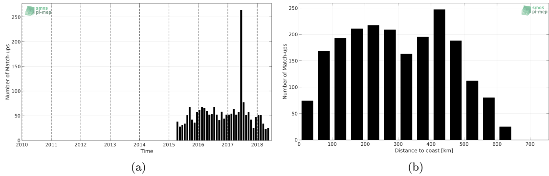
Figure 1: Number of match-ups between Argo and SMAP-L2-JPL-V4 SSS as a function of time (a) and as function of the distance to coast (b) over the Bay of Bengal Pi-MEP region and for the full satellite product period.
