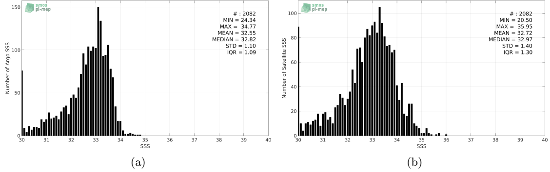
Figure 2: Histograms of SSS from Argo (a) and SMAP-L2-JPL-V4 (b) considering all match-up pairs per bins of 0.1 over the Bay of Bengal Pi-MEP region and for the full satellite product period.
