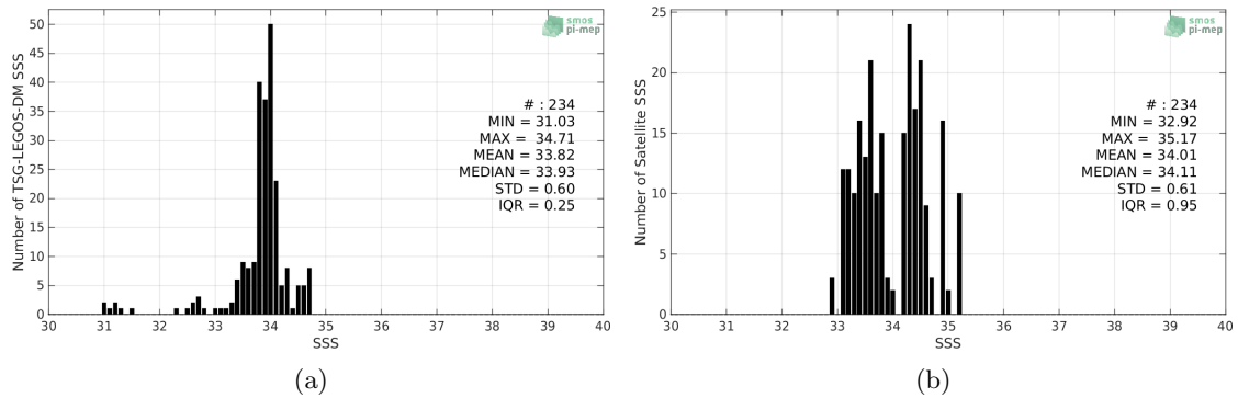
Figure 2: Histograms of SSS from TSG-LEGOS-DM (a) and SMAP-L2-JPL-V4.2 (b) considering all match-up pairs per bins of 0.1 over the Bay of Bengal Pi-MEP region and for the full satellite product period.
