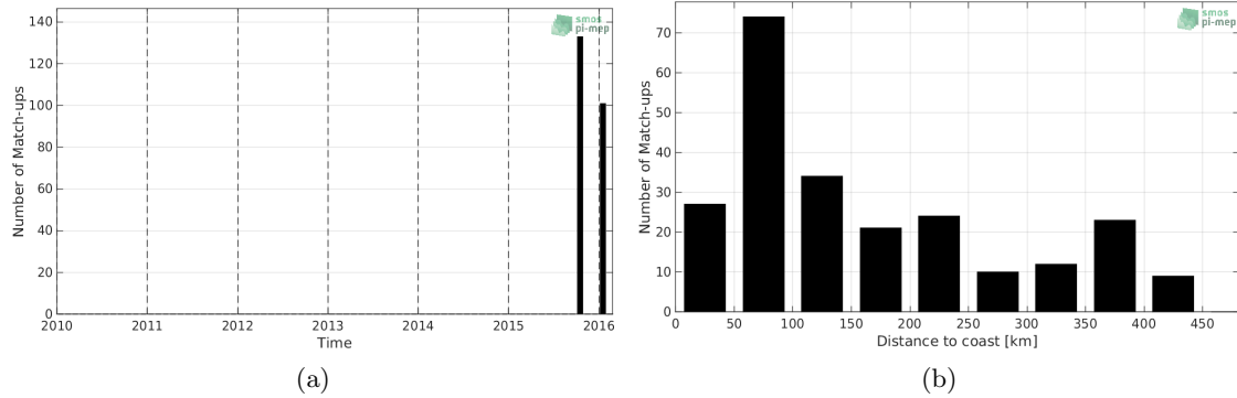
Figure 1: Number of match-ups between TSG-LEGOS-DM and SMAP-L2-JPL-V4.2 SSS as a function of time (a) and as function of the distance to coast (b) over the Bay of Bengal Pi-MEP region and for the full satellite product period.
