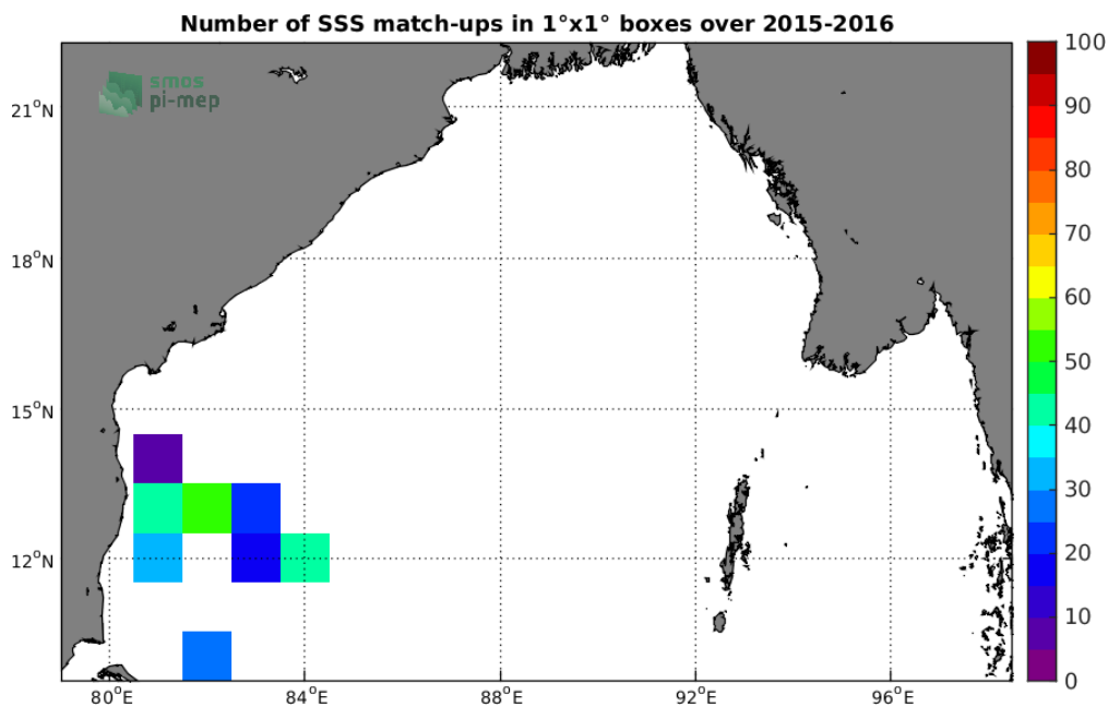
Figure 4: Number of SSS match-ups between TSG-LEGOS-DM SSS and the SMAP-L2-JPL-V4.2 SSS product for the Bay of Bengal Pi-MEP region over 1^\circ \times 1^\circ boxes and for the full satellite product period.
