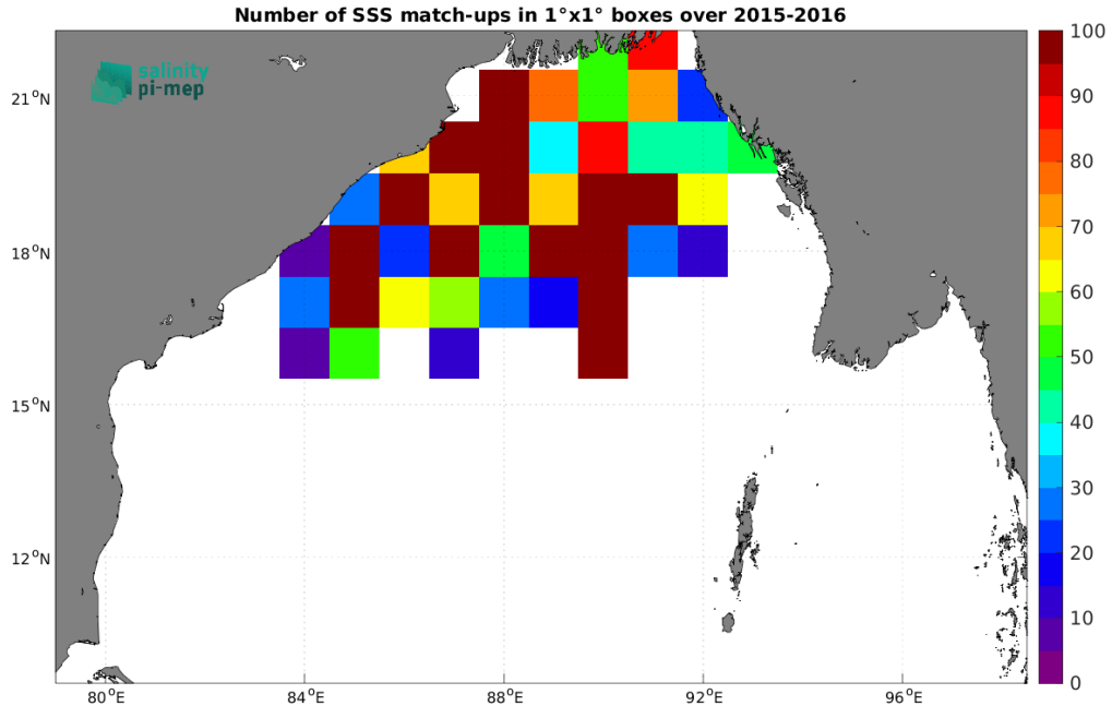
Figure 4: Number of SSS match-ups between Surface drifters SSS and the ISAS SSS product for the Bay of Bengal Pi-MEP region over 1^\circ \times 1^\circ boxes and for the full satellite product period.
