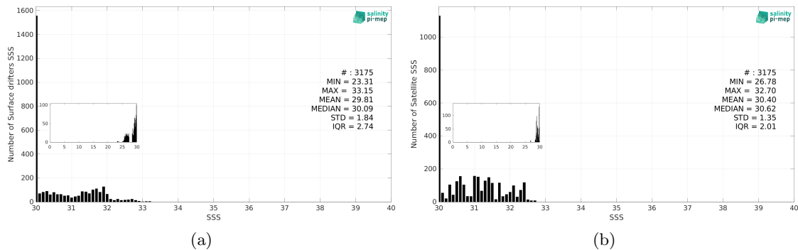
Figure 3: Histograms of SSS from Surface drifters (a) and ISAS (b) considering all match-up pairs per bins of 0.1 over the Bay of Bengal Pi-MEP region and for the full satellite product period.
