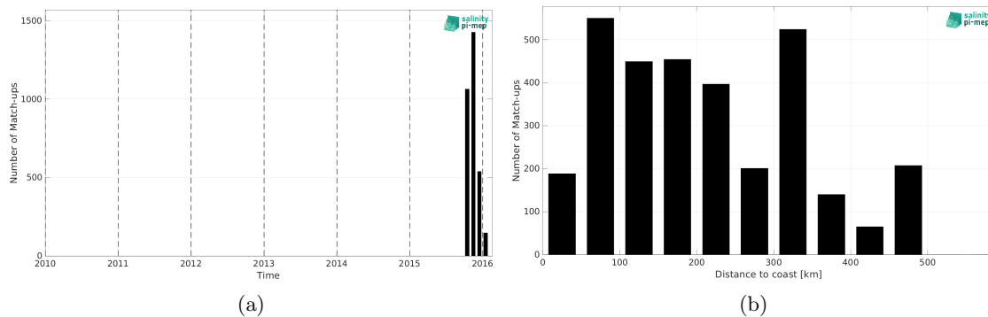
Figure 2: Number of match-ups between Surface drifters and ISAS SSS as a function of time (a) and as function of the distance to coast (b) over the Bay of Bengal Pi-MEP region and for the full satellite product period.
