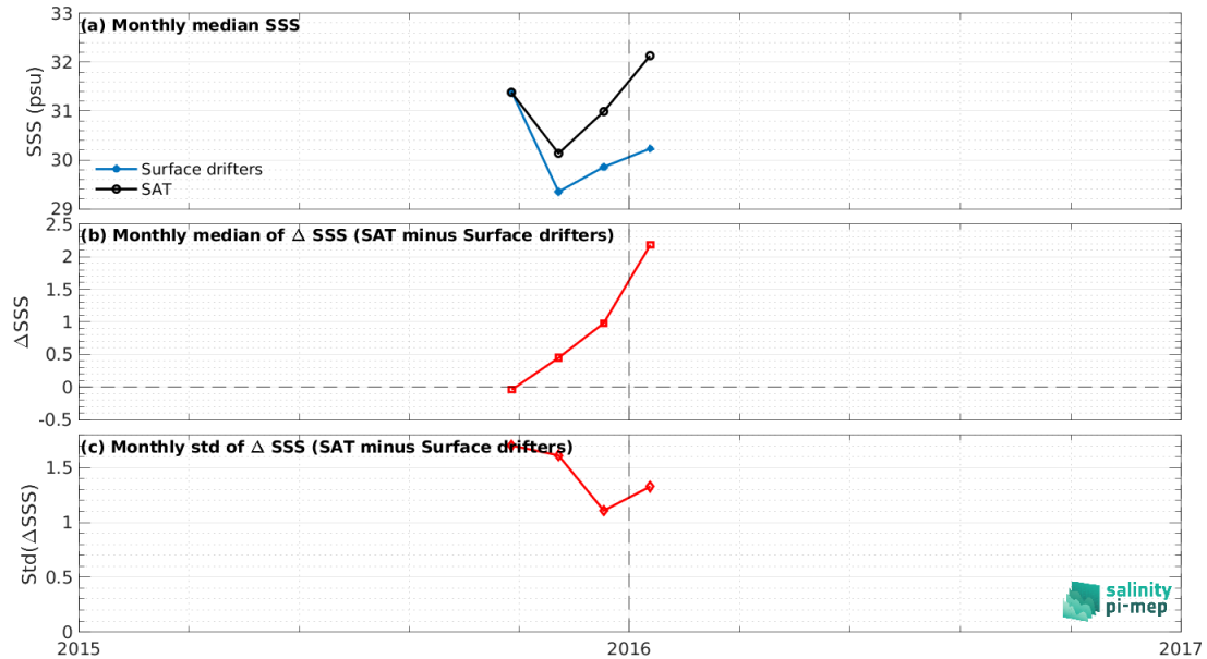
Figure 7: Time series of the monthly median SSS (top), median of \Delta\text{SSS} (Satellite - Surface drifters) and Std of \Delta\text{SSS} (Satellite - Surface drifters) over the Bay of Bengal Pi-MEP region considering all match-ups collected by the Pi-MEP.
