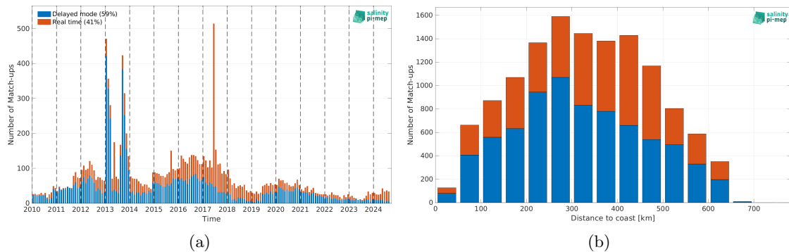
Figure 2: Number of match-ups between Argo and ISAS v7 - Monthly (Ifremer-LOPS-CMEMS) SSS as a function of time (a) and as function of the distance to coast (b) over the Bay of Bengal Pi-MEP region and for the full satellite product period.
