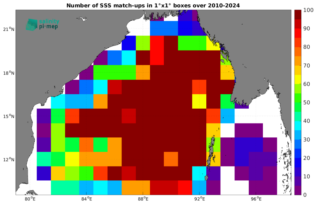
Figure 5: Number of SSS match-ups between Argo SSS and the ISAS v7 - Monthly (Ifremer-LOPS-CMEMS) SSS product for the Bay of Bengal Pi-MEP region over 1^\circ \times 1^\circ boxes and for the full satellite product period.
