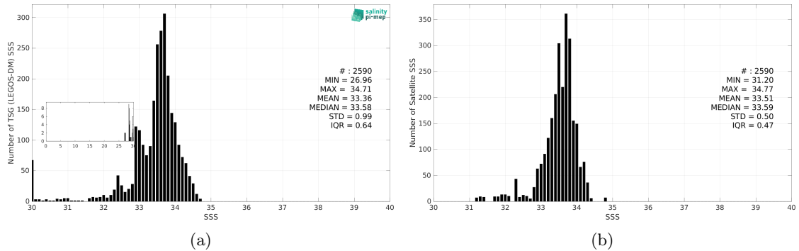
Figure 3: Histograms of SSS from TSG (LEGOS-DM) (a) and CCI SSS L4 Merged-OI v5.5 - 7-day running (ESA) (b) considering all match-up pairs per bins of 0.1 over the Bay of Bengal Pi-MEP region and for the full satellite product period.
