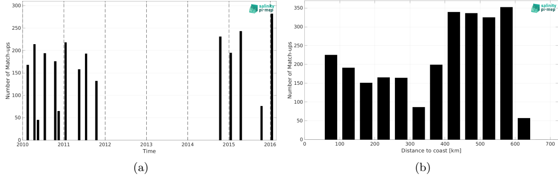
Figure 2: Number of match-ups between TSG (LEGOS-DM) and CCI SSS L4 Merged-OI v5.5 - 7-day running (ESA) SSS as a function of time (a) and as function of the distance to coast (b) over the Bay of Bengal Pi-MEP region and for the full satellite product period.
