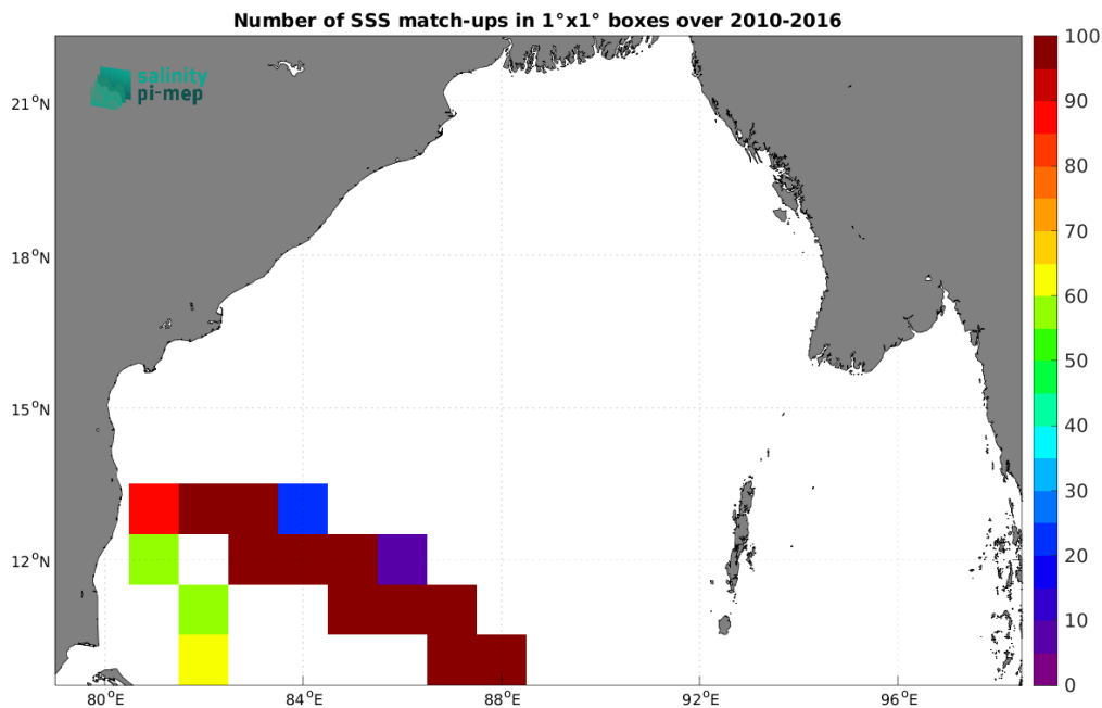
Figure 5: Number of SSS match-ups between TSG (LEGOS-DM) SSS and the CCI SSS L4 Merged-OI v5.5 - 7-day running (ESA) SSS product for the Bay of Bengal Pi-MEP region over 1^\circ \times 1^\circ boxes and for the full satellite product period.
