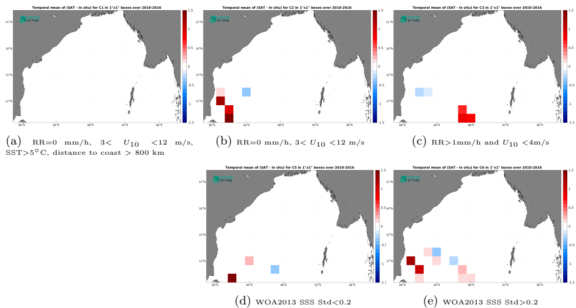
Figure 14: Temporal mean gridded over spatial boxes of size 1^\circ \times 1^\circ of \Delta\text{SSS} (CCI SSS L4 Merged-OI v5.5 - 7-day running (ESA) - TSG (LEGOS-DM)) for 5 different subdatasets corresponding to:RR=0 mm/h, 3 < U_{10} < 12 m/s, SST >5^\circ\text{C} , distance to coast > 800 km (a), RR=0 mm/h, 3 < U_{10} < 12 m/s (b), RR >1 mm/h and U_{10} < 4 m/s (c), WOA2013 SSS Std <0.2 (d), WOA2013 SSS Std >0.2 (e).
