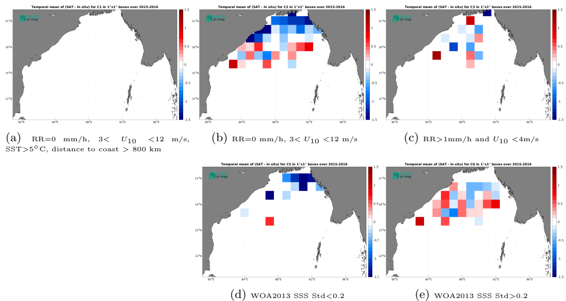
Figure 13: Temporal mean gridded over spatial boxes of size 1^\circ \times 1^\circ of \Delta\text{SSS} (CCI SSS L4 Merged-OI v5.5 - 7-day running (ESA) - Surface drifters) for 5 different subdatasets corresponding to:RR=0 mm/h, 3 < U_{10} < 12 m/s, SST >5^\circ\text{C} , distance to coast > 800 km (a), RR=0 mm/h, 3 < U_{10} < 12 m/s (b), RR >1 mm/h and U_{10} < 4 m/s (c), WOA2013 SSS Std <0.2 (d), WOA2013 SSS Std >0.2 (e).
