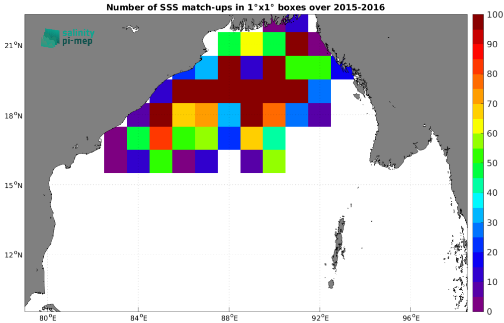
Figure 4: Number of SSS match-ups between Surface drifters SSS and the CCI SSS L4 Merged-OI v5.5 - 7-day running (ESA) SSS product for the Bay of Bengal Pi-MEP region over 1^\circ \times 1^\circ boxes and for the full satellite product period.
