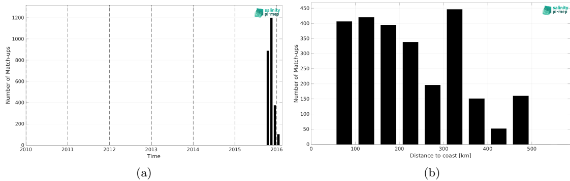
Figure 2: Number of match-ups between Surface drifters and CCI SSS L4 Merged-OI v5.5 - 7-day running (ESA) SSS as a function of time (a) and as function of the distance to coast (b) over the Bay of Bengal Pi-MEP region and for the full satellite product period.
