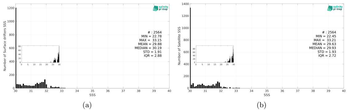
Figure 3: Histograms of SSS from Surface drifters (a) and CCI SSS L4 Merged-OI v5.5 - 7-day running (ESA) (b) considering all match-up pairs per bins of 0.1 over the Bay of Bengal Pi-MEP region and for the full satellite product period.
