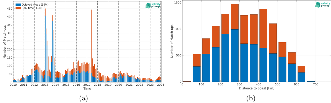
Figure 2: Number of match-ups between Argo and CCI SSS L4 Merged-OI v5.5 - 7-day running (ESA) SSS as a function of time (a) and as function of the distance to coast (b) over the Bay of Bengal Pi-MEP region and for the full satellite product period.
