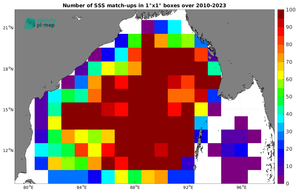
Figure 5: Number of SSS match-ups between Argo SSS and the CCI SSS L4 Merged-OI v5.5 - 7-day running (ESA) SSS product for the Bay of Bengal Pi-MEP region over 1^\circ \times 1^\circ boxes and for the full satellite product period.
