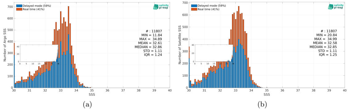
Figure 3: Histograms of SSS from Argo (a) and CCI SSS L4 Merged-OI v5.5 - 7-day running (ESA) (b) considering all match-up pairs per bins of 0.1 over the Bay of Bengal Pi-MEP region and for the full satellite product period.
