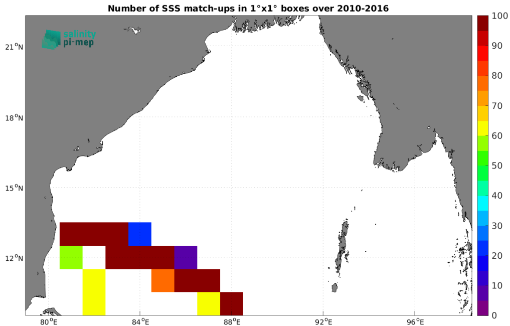
Figure 5: Number of SSS match-ups between TSG (LEGOS-DM) SSS and the CCI SSS L4 Merged-OI v5.5 - 30-day running (ESA) SSS product for the Bay of Bengal Pi-MEP region over 1^\circ \times 1^\circ boxes and for the full satellite product period.
