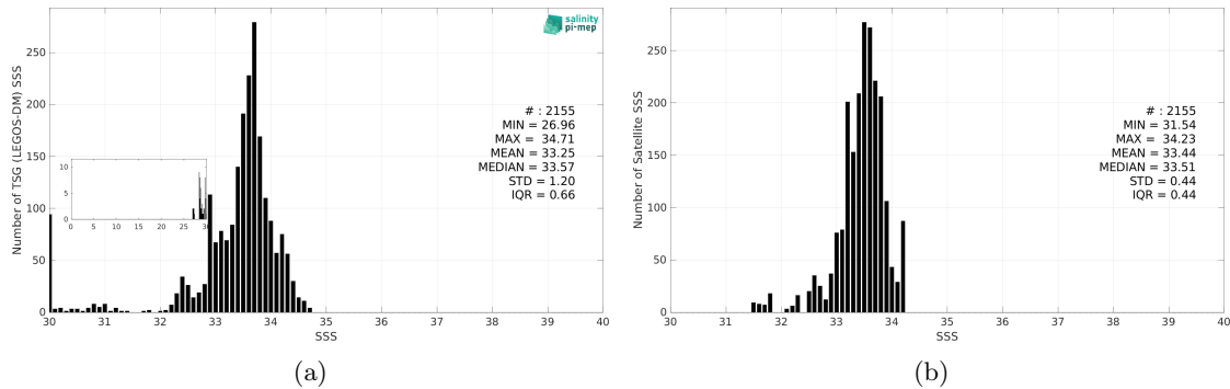
Figure 3: Histograms of SSS from TSG (LEGOS-DM) (a) and CCI SSS L4 Merged-OI v5.5 - 30-day running (ESA) (b) considering all match-up pairs per bins of 0.1 over the Bay of Bengal Pi-MEP region and for the full satellite product period.
