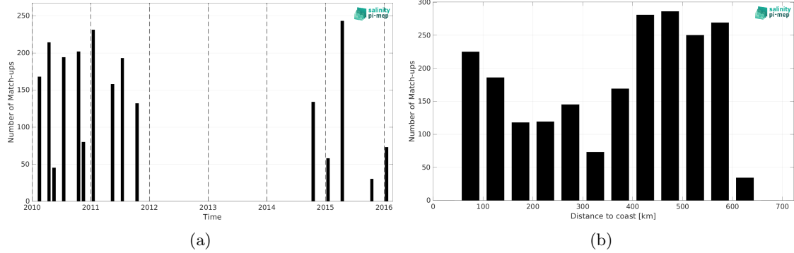
Figure 2: Number of match-ups between TSG (LEGOS-DM) and CCI SSS L4 Merged-OI v5.5 - 30-day running (ESA) SSS as a function of time (a) and as function of the distance to coast (b) over the Bay of Bengal Pi-MEP region and for the full satellite product period.
