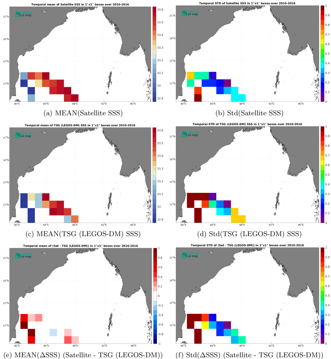
Figure 7: Temporal mean (left) and Std (right) of SSS from CCI SSS L4 Merged-OI v5.5 - 30-day running (ESA) (top), TSG (LEGOS-DM) (middle), and of \Delta SSS (Satellite - TSG (LEGOS-DM)). Only match-up pairs are used to generate these maps.
