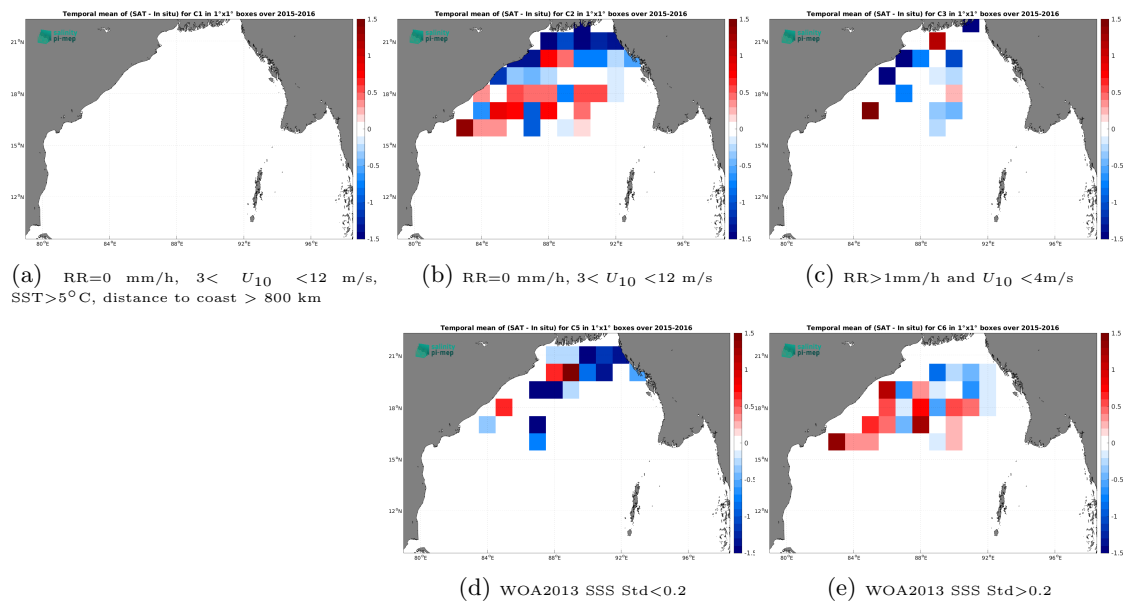
Figure 13: Temporal mean gridded over spatial boxes of size 1^\circ \times 1^\circ of \Delta\text{SSS} (CCI SSS L4 Merged-OI v5.5 - 30-day running (ESA) - Surface drifters) for 5 different subdatasets corresponding to:RR=0 mm/h, 3 < U_{10} < 12 m/s, SST > 5^\circ\text{C} , distance to coast > 800 km (a), RR=0 mm/h, 3 < U_{10} < 12 m/s (b), RR > 1 mm/h and U_{10} < 4 m/s (c), WOA2013 SSS Std < 0.2 (d), WOA2013 SSS Std > 0.2 (e).
