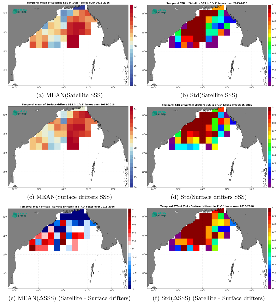
Figure 6: Temporal mean (left) and Std (right) of SSS from CCI SSS L4 Merged-OI v5.5 - 30-day running (ESA) (top), Surface drifters (middle), and of \Delta SSS (Satellite - Surface drifters). Only match-up pairs are used to generate these maps.
