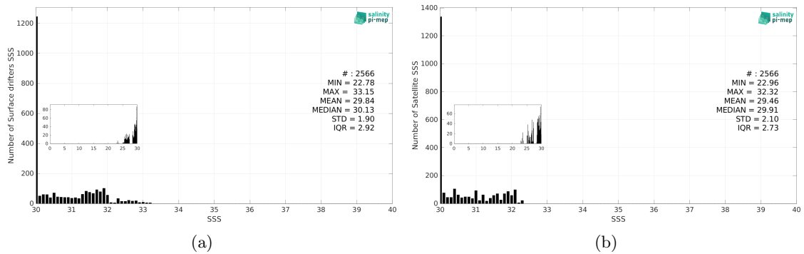
Figure 3: Histograms of SSS from Surface drifters (a) and CCI SSS L4 Merged-OI v5.5 - 30-day running (ESA) (b) considering all match-up pairs per bins of 0.1 over the Bay of Bengal Pi-MEP region and for the full satellite product period.
