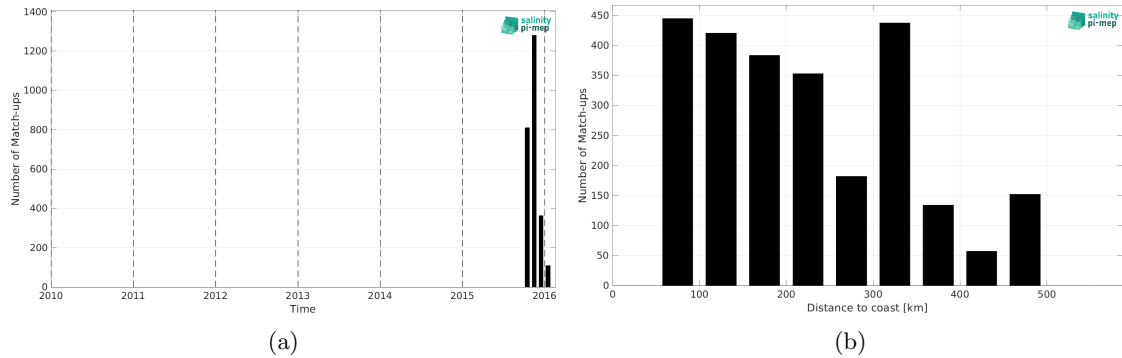
Figure 2: Number of match-ups between Surface drifters and CCI SSS L4 Merged-OI v5.5 - 30-day running (ESA) SSS as a function of time (a) and as function of the distance to coast (b) over the Bay of Bengal Pi-MEP region and for the full satellite product period.
