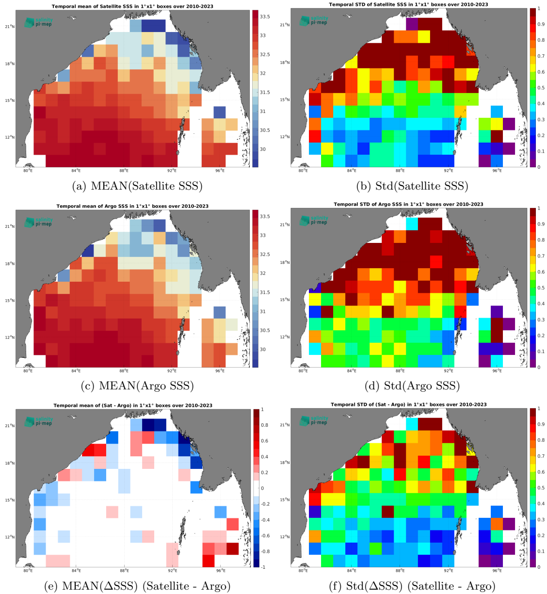
Figure 7: Temporal mean (left) and Std (right) of SSS from CCI SSS L4 Merged-OI v5.5 - 30-day running (ESA) (top), Argo (middle), and of \Delta SSS (Satellite - Argo). Only match-up pairs are used to generate these maps.
