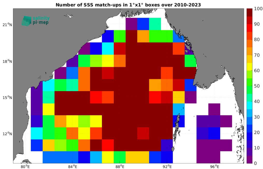
Figure 5: Number of SSS match-ups between Argo SSS and the CCI SSS L4 Merged-OI v5.5 - 30-day running (ESA) SSS product for the Bay of Bengal Pi-MEP region over 1^\circ \times 1^\circ boxes and for the full satellite product period.
