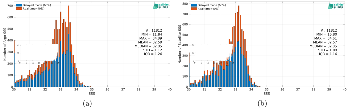
Figure 3: Histograms of SSS from Argo (a) and CCI SSS L4 Merged-OI v5.5 - 30-day running (ESA) (b) considering all match-up pairs per bins of 0.1 over the Bay of Bengal Pi-MEP region and for the full satellite product period.
