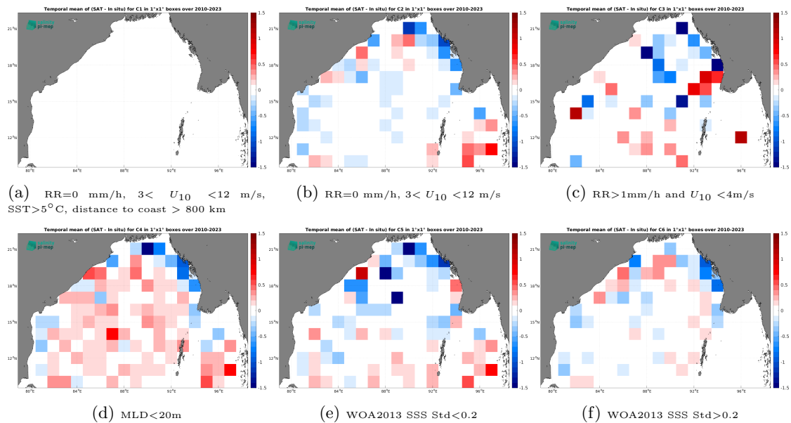
Figure 14: Temporal mean gridded over spatial boxes of size 1^\circ \times 1^\circ of \Delta SSS (CCI SSS L4 Merged-OI v5.5 - 30-day running (ESA) - Argo) for 6 different subdatasets corresponding to:RR=0 mm/h, 3 < U_{10} < 12 m/s, SST > 5^\circ\text{C} , distance to coast > 800 km (a), RR=0 mm/h, 3 < U_{10} < 12 m/s (b), RR > 1 mm/h and U_{10} < 4 m/s (c),MLD < 20 m (d),WOA2013 SSS Std < 0.2 (e),WOA2013 SSS Std > 0.2 (f).
