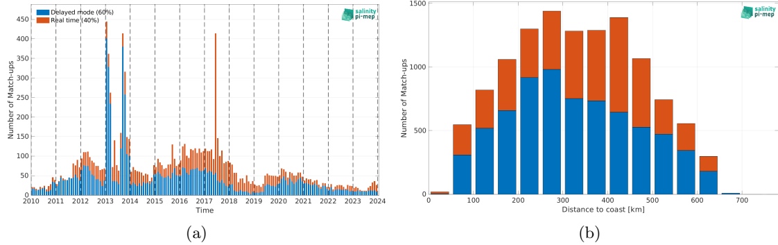
Figure 2: Number of match-ups between Argo and CCI SSS L4 Merged-OI v5.5 - 30-day running (ESA) SSS as a function of time (a) and as function of the distance to coast (b) over the Bay of Bengal Pi-MEP region and for the full satellite product period.
