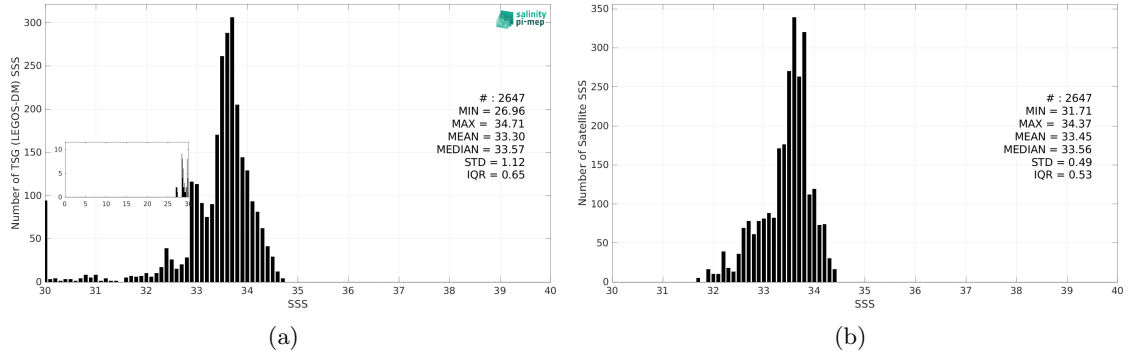
Figure 3: Histograms of SSS from TSG (LEGOS-DM) (a) and CCI SSS L4 Merged-OI v4.41 - 7-day running (ESA) (b) considering all match-up pairs per bins of 0.1 over the Bay of Bengal Pi-MEP region and for the full satellite product period.
