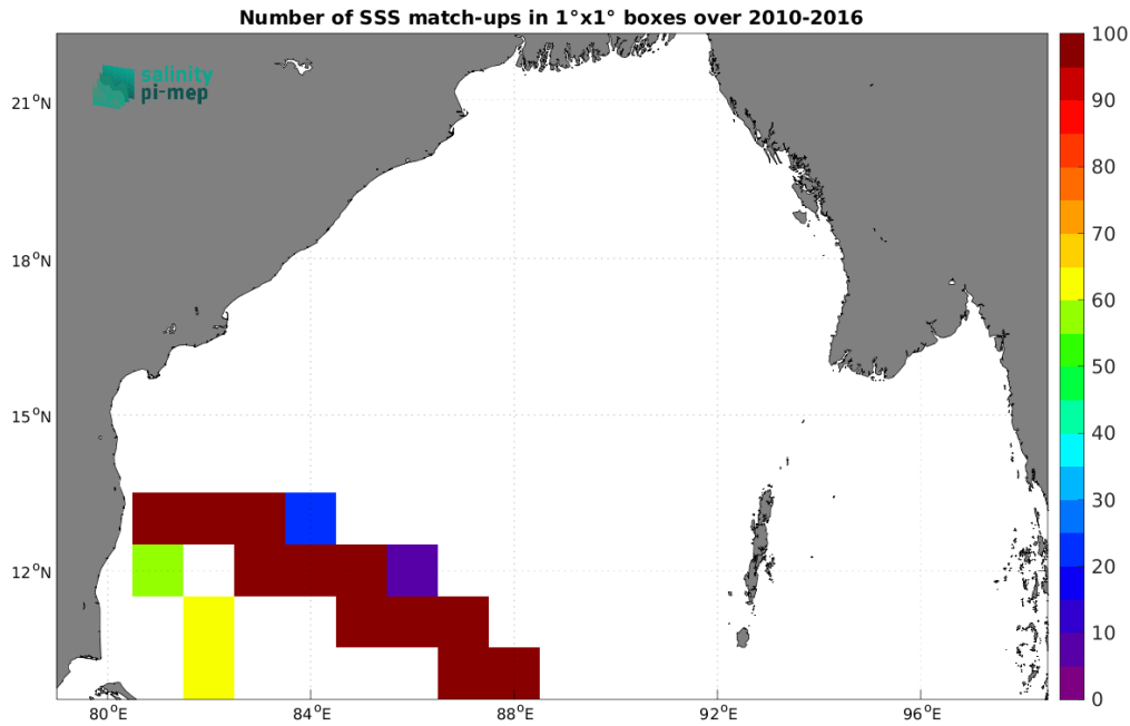
Figure 5: Number of SSS match-ups between TSG (LEGOS-DM) SSS and the CCI SSS L4 Merged-OI v4.41 - 7-day running (ESA) SSS product for the Bay of Bengal Pi-MEP region over 1^\circ \times 1^\circ boxes and for the full satellite product period.
