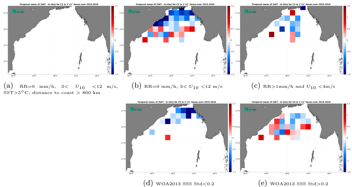
Figure 13: Temporal mean gridded over spatial boxes of size 1^\circ \times 1^\circ of \Delta\text{SSS} (CCI SSS L4 Merged-OI v4.41 - 7-day running (ESA) - Surface drifters) for 5 different subdatasets corresponding to:RR=0 mm/h, 3 < U_{10} < 12 m/s, SST >5^\circ\text{C} , distance to coast > 800 km (a), RR=0 mm/h, 3 < U_{10} < 12 m/s (b), RR >1 mm/h and U_{10} < 4 m/s (c), WOA2013 SSS Std <0.2 (d), WOA2013 SSS Std >0.2 (e).
