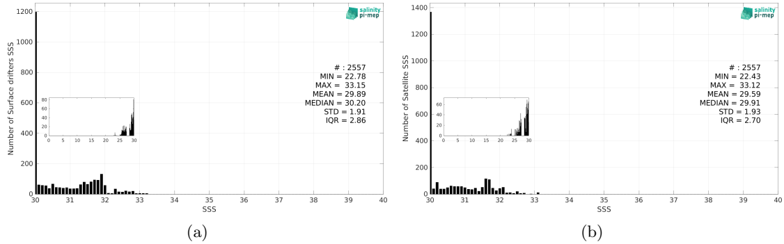
Figure 3: Histograms of SSS from Surface drifters (a) and CCI SSS L4 Merged-OI v4.41 - 7-day running (ESA) (b) considering all match-up pairs per bins of 0.1 over the Bay of Bengal Pi-MEP region and for the full satellite product period.
