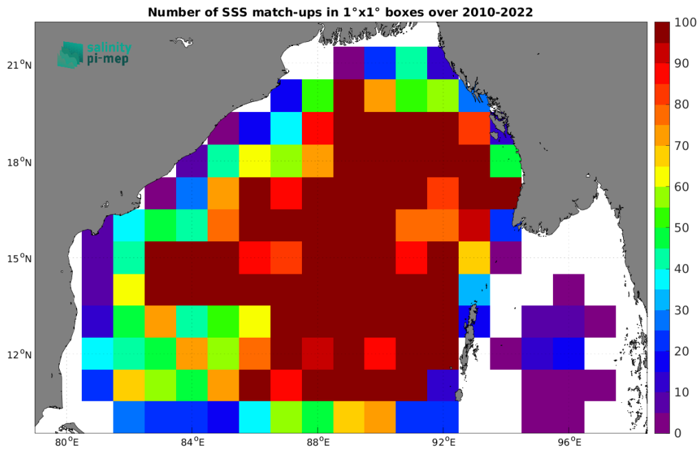
Figure 5: Number of SSS match-ups between Argo SSS and the CCI SSS L4 Merged-OI v4.41 - 7-day running (ESA) SSS product for the Bay of Bengal Pi-MEP region over 1^{\circ} \times 1^{\circ} boxes and for the full satellite product period.
