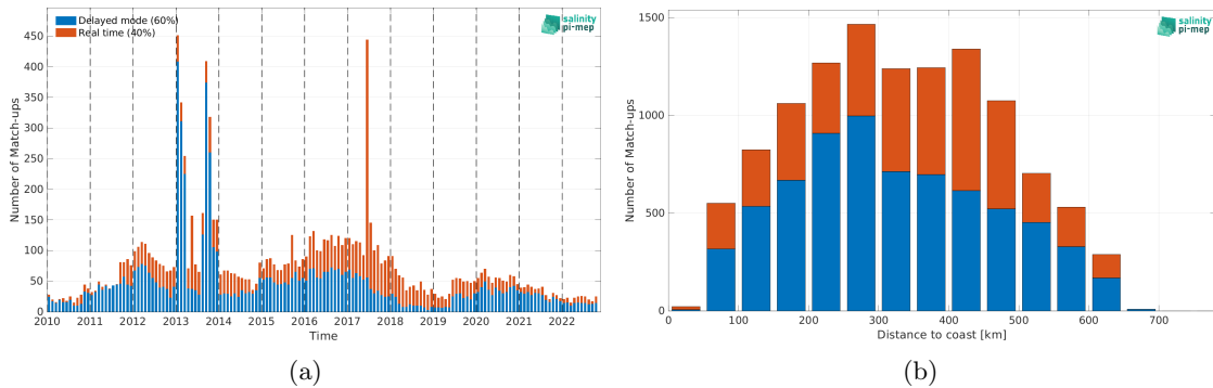
Figure 2: Number of match-ups between Argo and CCI SSS L4 Merged-OI v4.41 - 7-day running (ESA) SSS as a function of time (a) and as function of the distance to coast (b) over the Bay of Bengal Pi-MEP region and for the full satellite product period.
