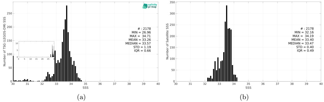
Figure 3: Histograms of SSS from TSG (LEGOS-DM) (a) and CCI SSS L4 Merged-OI v4.41 - 30-day running (ESA) (b) considering all match-up pairs per bins of 0.1 over the Bay of Bengal Pi-MEP region and for the full satellite product period.
