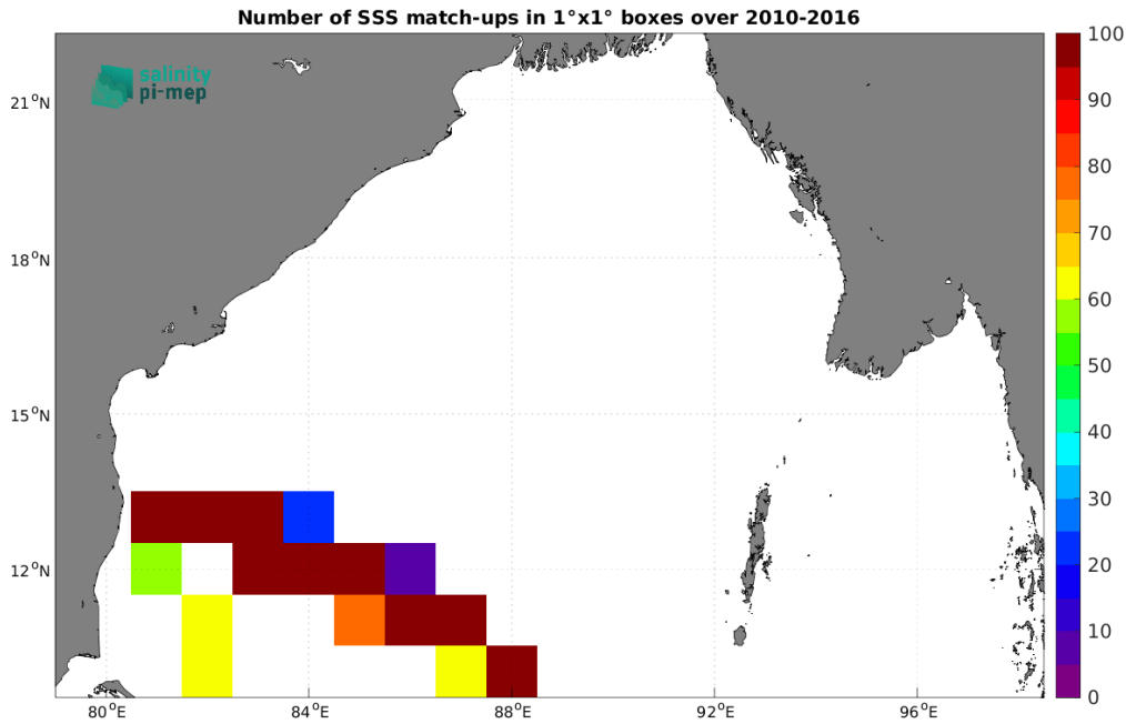
Figure 5: Number of SSS match-ups between TSG (LEGOS-DM) SSS and the CCI SSS L4 Merged-OI v4.41 - 30-day running (ESA) SSS product for the Bay of Bengal Pi-MEP region over 1^{\circ} \times 1^{\circ} boxes and for the full satellite product period.
