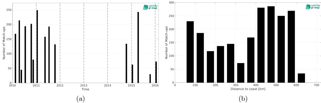
Figure 2: Number of match-ups between TSG (LEGOS-DM) and CCI SSS L4 Merged-OI v4.41 - 30-day running (ESA) SSS as a function of time (a) and as function of the distance to coast (b) over the Bay of Bengal Pi-MEP region and for the full satellite product period.
