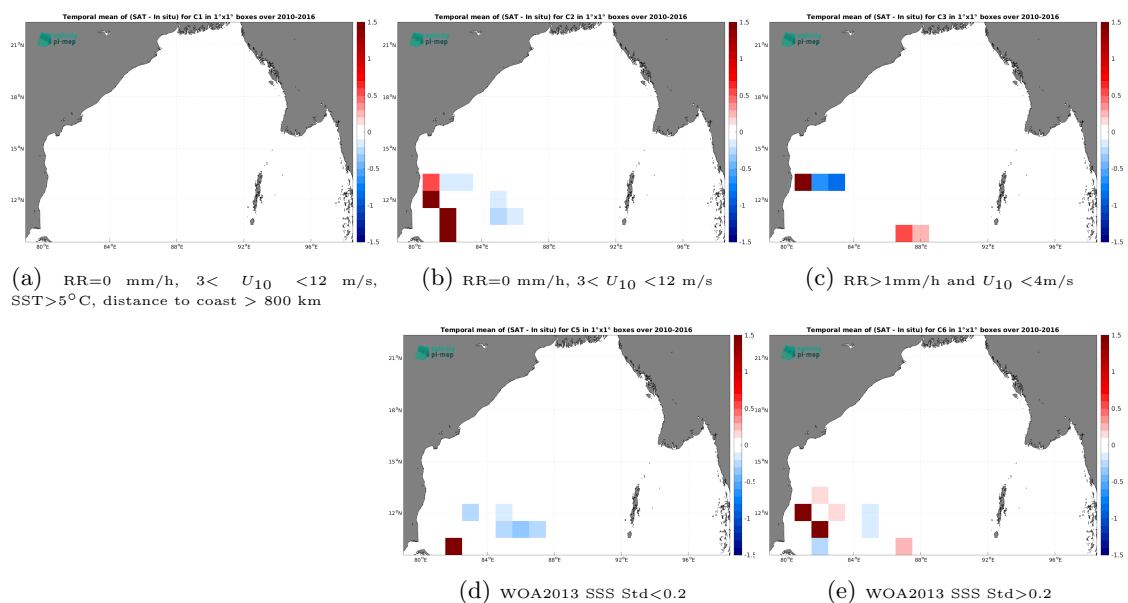
Figure 14: Temporal mean gridded over spatial boxes of size 1^\circ \times 1^\circ of \Delta\text{SSS} (CCI SSS L4 Merged-OI v4.41 - 30-day running (ESA) - TSG (LEGOS-DM)) for 5 different subdatasets corresponding to:RR=0 mm/h, 3 < U_{10} < 12 m/s, SST >5^\circ\text{C} , distance to coast > 800 km (a), RR=0 mm/h, 3 < U_{10} < 12 m/s (b), RR >1 mm/h and U_{10} < 4 m/s (c), WOA2013 SSS Std <0.2 (d), WOA2013 SSS Std >0.2 (e).
