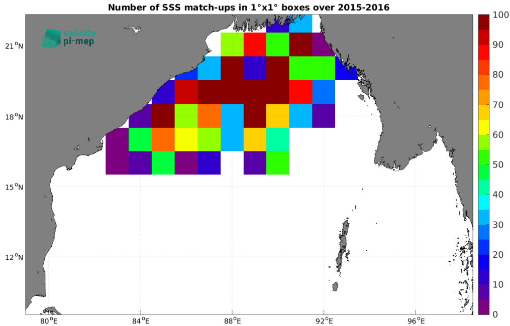
Figure 4: Number of SSS match-ups between Surface drifters SSS and the CCI SSS L4 Merged-OI v4.41 - 30-day running (ESA) SSS product for the Bay of Bengal Pi-MEP region over 1^\circ \times 1^\circ boxes and for the full satellite product period.
