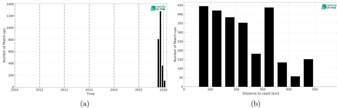
Figure 2: Number of match-ups between Surface drifters and CCI SSS L4 Merged-OI v4.41 - 30-day running (ESA) SSS as a function of time (a) and as function of the distance to coast (b) over the Bay of Bengal Pi-MEP region and for the full satellite product period.
