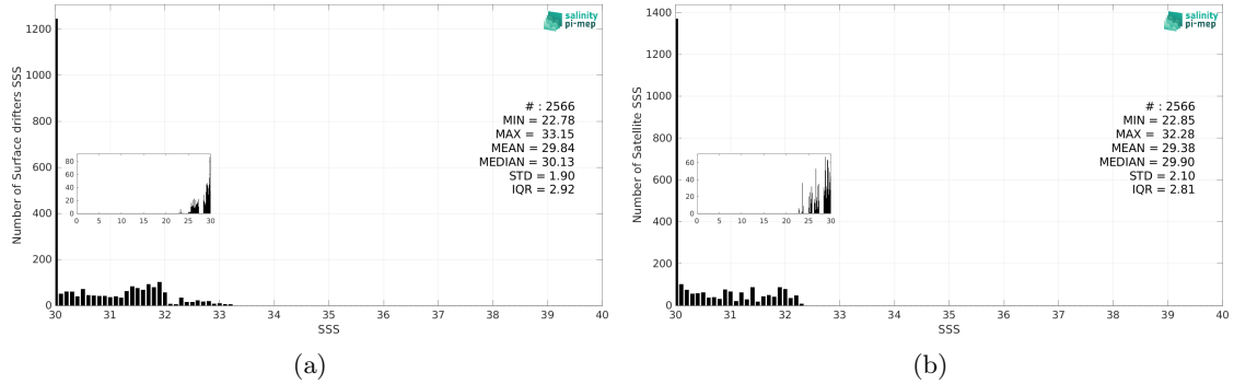
Figure 3: Histograms of SSS from Surface drifters (a) and CCI SSS L4 Merged-OI v4.41 - 30-day running (ESA) (b) considering all match-up pairs per bins of 0.1 over the Bay of Bengal Pi-MEP region and for the full satellite product period.
