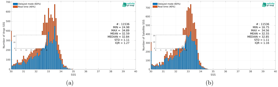
Figure 3: Histograms of SSS from Argo (a) and CCI SSS L4 Merged-OI v4.41 - 30-day running (ESA) (b) considering all match-up pairs per bins of 0.1 over the Bay of Bengal Pi-MEP region and for the full satellite product period.
