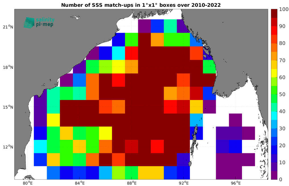
Figure 5: Number of SSS match-ups between Argo SSS and the CCI SSS L4 Merged-OI v4.41 - 30-day running (ESA) SSS product for the Bay of Bengal Pi-MEP region over 1^\circ \times 1^\circ boxes and for the full satellite product period.
