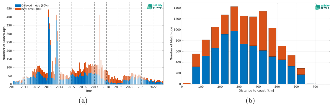
Figure 2: Number of match-ups between Argo and CCI SSS L4 Merged-OI v4.41 - 30-day running (ESA) SSS as a function of time (a) and as function of the distance to coast (b) over the Bay of Bengal Pi-MEP region and for the full satellite product period.
