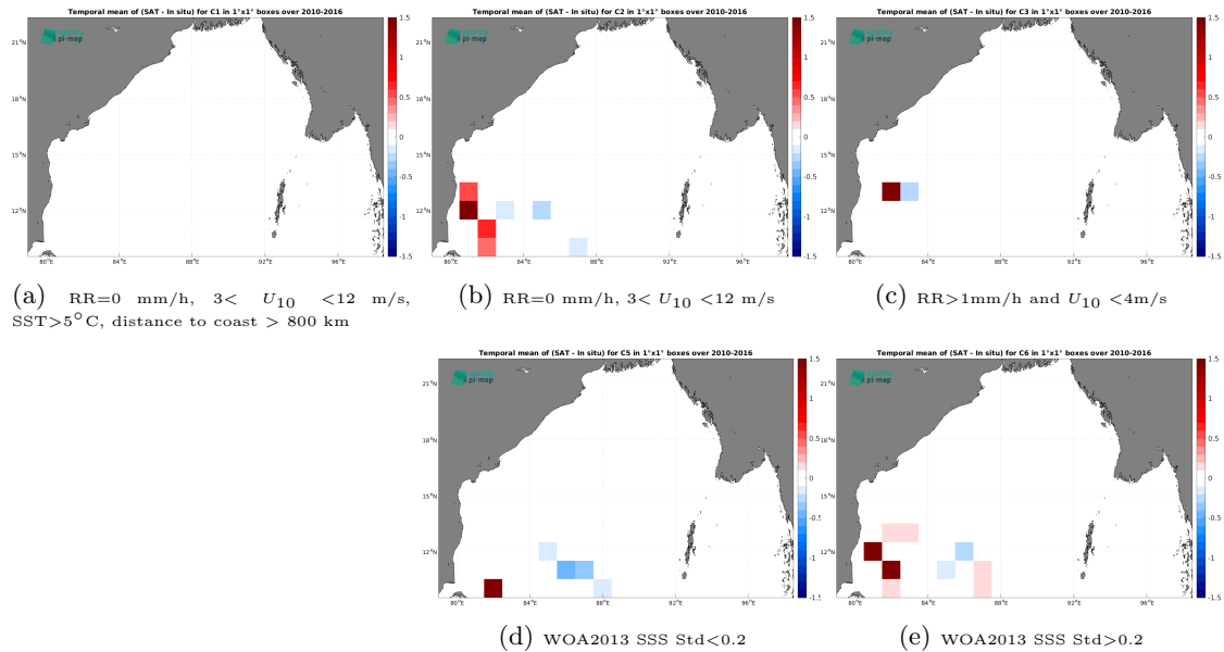
Figure 12: Temporal mean gridded over spatial boxes of size 1^{\circ}\times 1^{\circ} of \Delta\text{SSS} (CCI SSS L4 Merged-OI v4.4 - 7-day running (ESA) - TSG (LEGOS-DM)) for 5 different subdatasets corresponding to: RR=0 mm/h, 3 < U_{10} < 12 m/s, SST > 5^{\circ}\text{C} , distance to coast > 800 km (a), RR=0 mm/h, 3 < U_{10} < 12 m/s (b), RR > 1 mm/h and U_{10} < 4 m/s (c), WOA2013 SSS Std < 0.2 (d), WOA2013 SSS Std > 0.2 (e).
