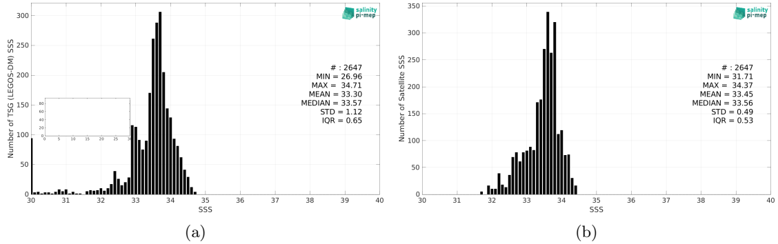
Figure 2: Histograms of SSS from TSG (LEGOS-DM) (a) and CCI SSS L4 Merged-OI v4.4 - 7-day running (ESA) (b) considering all match-up pairs per bins of 0.1 over the Bay of Bengal Pi-MEP region and for the full satellite product period.
