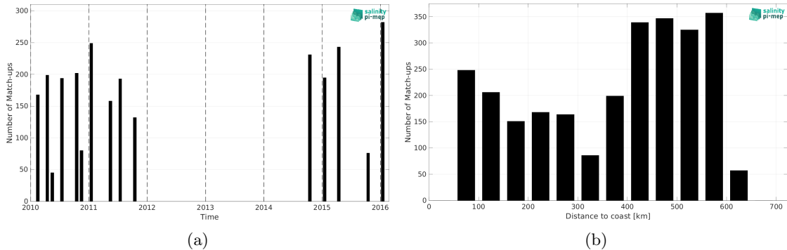
Figure 1: Number of match-ups between TSG (LEGOS-DM) and CCI SSS L4 Merged-OI v4.4 - 7-day running (ESA) SSS as a function of time (a) and as function of the distance to coast (b) over the Bay of Bengal Pi-MEP region and for the full satellite product period.
