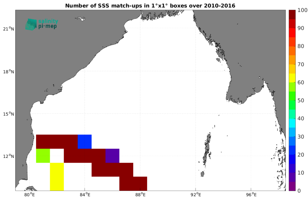
Figure 4: Number of SSS match-ups between TSG (LEGOS-DM) SSS and the CCI SSS L4 Merged-OI v4.4 - 7-day running (ESA) SSS product for the Bay of Bengal Pi-MEP region over 1^\circ \times 1^\circ boxes and for the full satellite product period.
