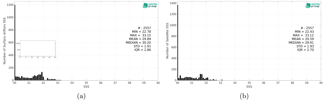
Figure 2: Histograms of SSS from Surface drifters (a) and CCI SSS L4 Merged-OI v4.4 - 7-day running (ESA) (b) considering all match-up pairs per bins of 0.1 over the Bay of Bengal Pi-MEP region and for the full satellite product period.
