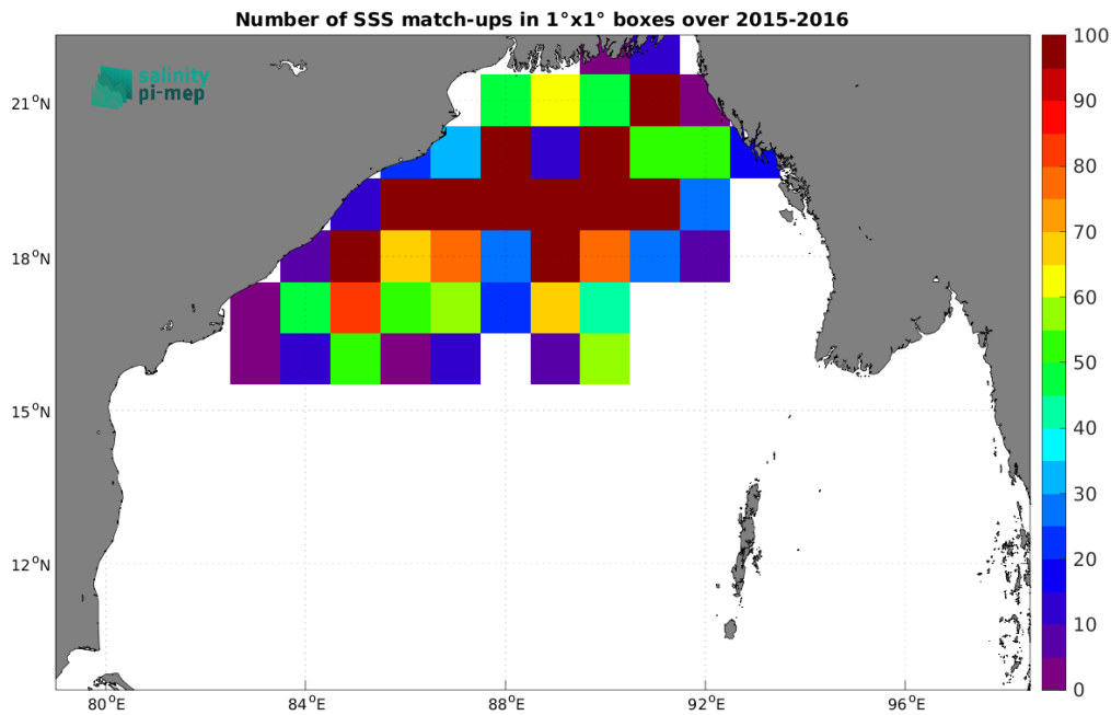
Figure 3: Number of SSS match-ups between Surface drifters SSS and the CCI SSS L4 Merged-OI v4.4 - 7-day running (ESA) SSS product for the Bay of Bengal Pi-MEP region over 1^\circ \times 1^\circ boxes and for the full satellite product period.
