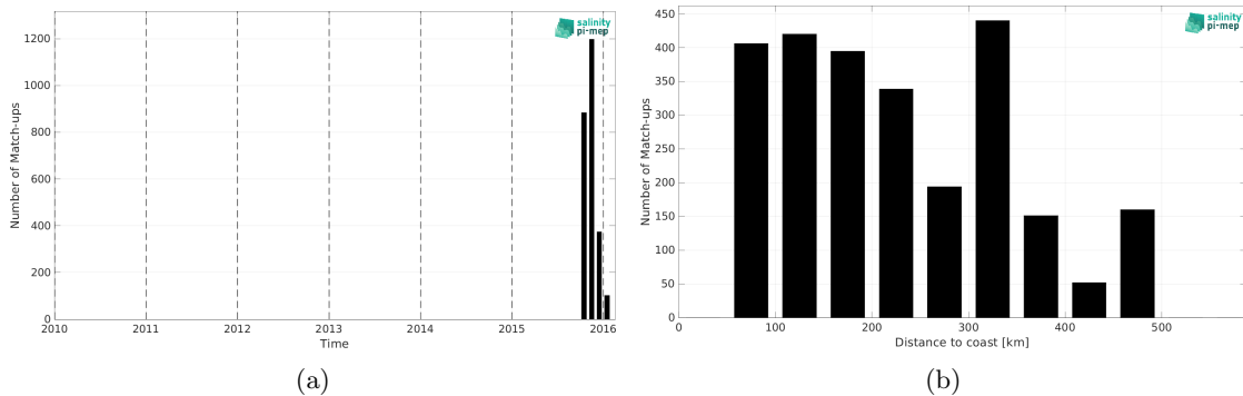
Figure 1: Number of match-ups between Surface drifters and CCI SSS L4 Merged-OI v4.4 - 7-day running (ESA) SSS as a function of time (a) and as function of the distance to coast (b) over the Bay of Bengal Pi-MEP region and for the full satellite product period.
