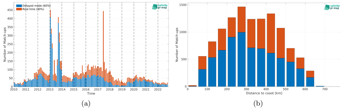
Figure 1: Number of match-ups between Argo and CCI SSS L4 Merged-OI v4.4 - 7-day running (ESA) SSS as a function of time (a) and as function of the distance to coast (b) over the Bay of Bengal Pi-MEP region and for the full satellite product period.
