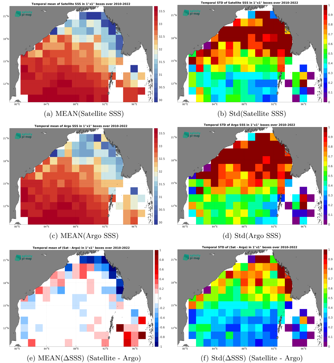
Figure 6: Temporal mean (left) and Std (right) of SSS from CCI SSS L4 Merged-OI v4.4 - 7-day running (ESA) (top), Argo (middle), and of \Delta SSS (Satellite - Argo). Only match-up pairs are used to generate these maps.
