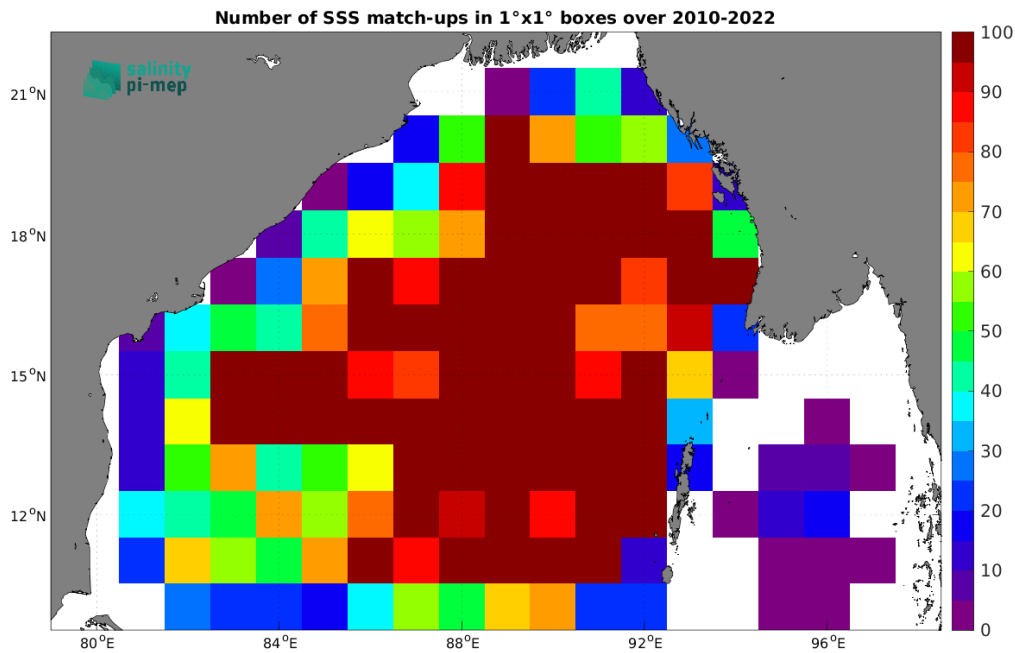
Figure 4: Number of SSS match-ups between Argo SSS and the CCI SSS L4 Merged-OI v4.4 - 7-day running (ESA) SSS product for the Bay of Bengal Pi-MEP region over 1^\circ \times 1^\circ boxes and for the full satellite product period.
