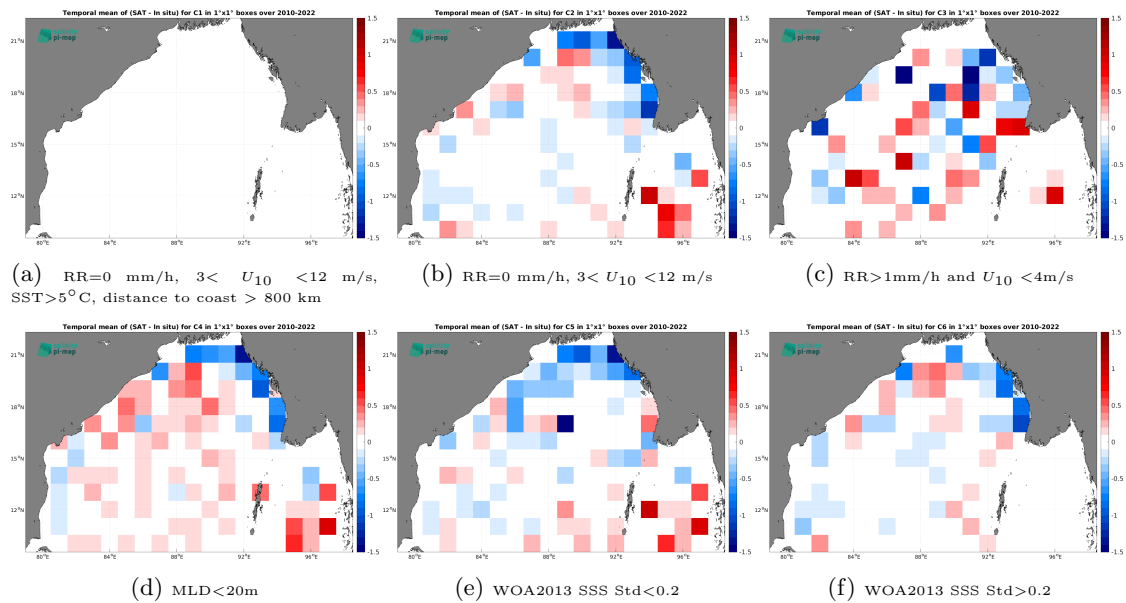
Figure 12: Temporal mean gridded over spatial boxes of size 1^\circ \times 1^\circ of \Delta SSS (CCI SSS L4 Merged-OI v4.4 - 7-day running (ESA) - Argo) for 6 different subdatasets corresponding to:RR=0 mm/h, 3 < U_{10} < 12 m/s, SST > 5^\circ\text{C} , distance to coast > 800 km (a), RR=0 mm/h, 3 < U_{10} < 12 m/s (b), RR > 1 mm/h and U_{10} < 4 m/s (c),MLD < 20 m (d),WOA2013 SSS Std < 0.2 (e),WOA2013 SSS Std > 0.2 (f).
