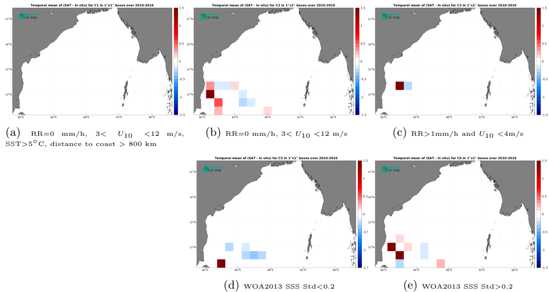
Figure 12: Temporal mean gridded over spatial boxes of size 1^{\circ}\times 1^{\circ} of \Delta\text{SSS} (CCI SSS L4 Merged-OI v4.4 - 30-day running (ESA) - TSG (LEGOS-DM)) for 5 different subdatasets corresponding to:RR=0 mm/h, 3 < U_{10} < 12 m/s, SST > 5^{\circ}\text{C} , distance to coast > 800 km (a), RR=0 mm/h, 3 < U_{10} < 12 m/s (b), RR > 1 mm/h and U_{10} < 4 m/s (c), WOA2013 SSS Std < 0.2 (d), WOA2013 SSS Std > 0.2 (e).
