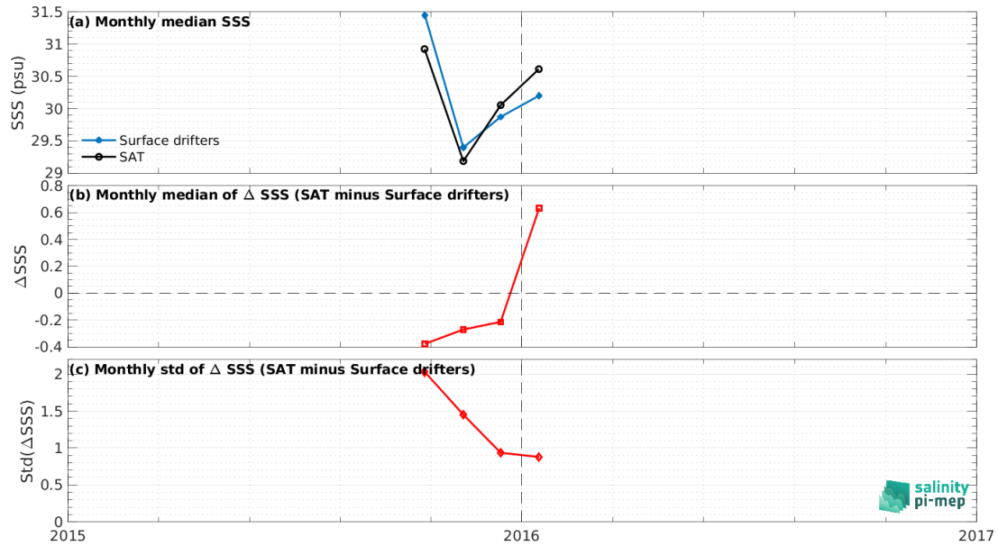
Figure 6: Time series of the monthly median SSS (top), median of \Delta\text{SSS} (Satellite - Surface drifters) and Std of \Delta\text{SSS} (Satellite - Surface drifters) over the Bay of Bengal Pi-MEP region considering all match-ups collected by the Pi-MEP.
