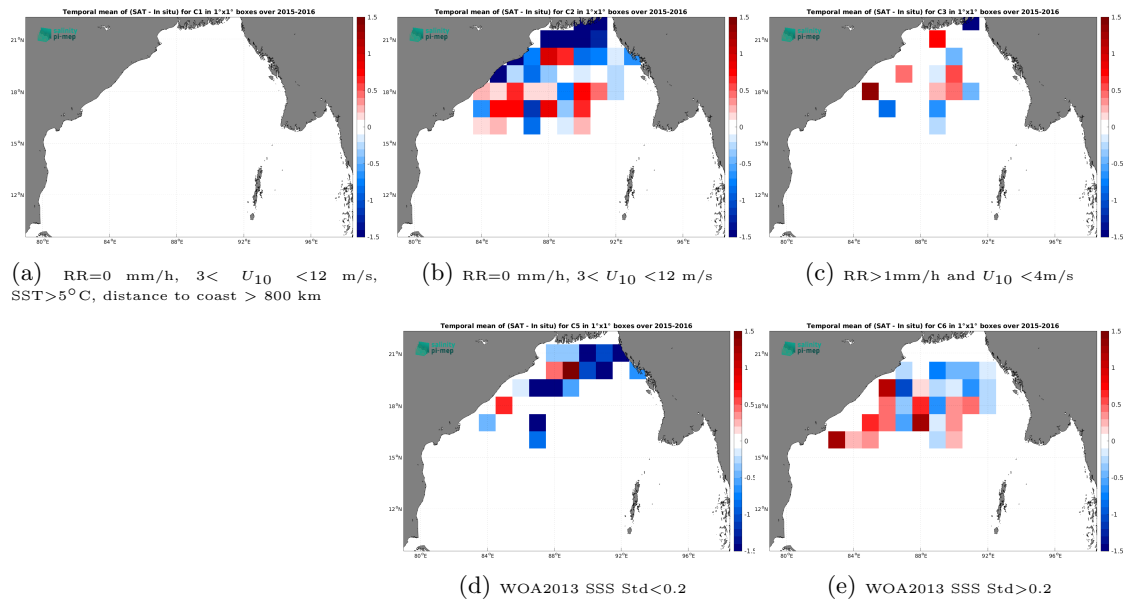
Figure 11: Temporal mean gridded over spatial boxes of size 1^\circ \times 1^\circ of \Delta\text{SSS} (CCI SSS L4 Merged-OI v4.4 - 30-day running (ESA) - Surface drifters) for 5 different subdatasets corresponding to:RR=0 mm/h, 3 < U_{10} < 12 m/s, SST >5^\circ\text{C} , distance to coast > 800 km (a), RR=0 mm/h, 3 < U_{10} < 12 m/s (b), RR >1 mm/h and U_{10} < 4 m/s (c), WOA2013 SSS Std <0.2 (d), WOA2013 SSS Std >0.2 (e).
