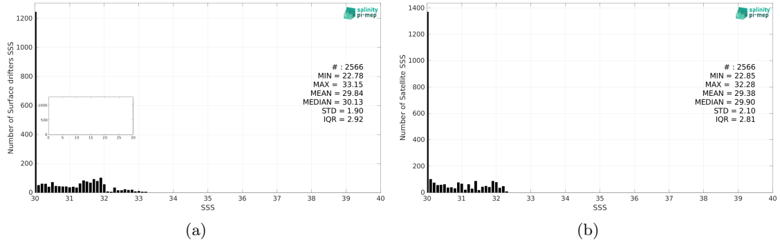
Figure 2: Histograms of SSS from Surface drifters (a) and CCI SSS L4 Merged-OI v4.4 - 30-day running (ESA) (b) considering all match-up pairs per bins of 0.1 over the Bay of Bengal Pi-MEP region and for the full satellite product period.
