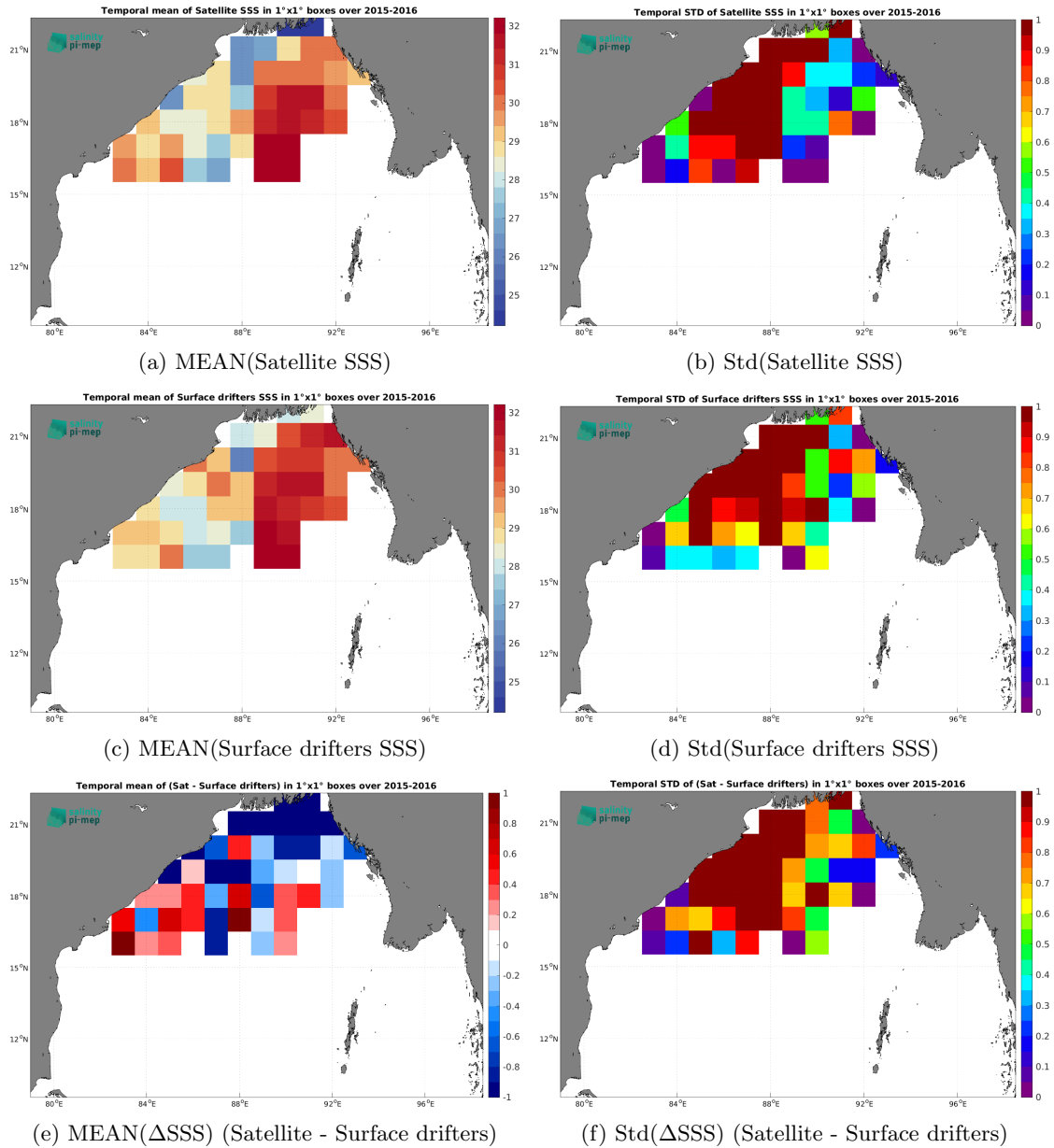
Figure 5: Temporal mean (left) and Std (right) of SSS from CCI SSS L4 Merged-OI v4.4 - 30-day running (ESA) (top), Surface drifters (middle), and of \Delta SSS (Satellite - Surface drifters). Only match-up pairs are used to generate these maps.
