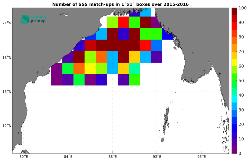
Figure 3: Number of SSS match-ups between Surface drifters SSS and the CCI SSS L4 Merged-OI v4.4 - 30-day running (ESA) SSS product for the Bay of Bengal Pi-MEP region over 1^\circ \times 1^\circ boxes and for the full satellite product period.
