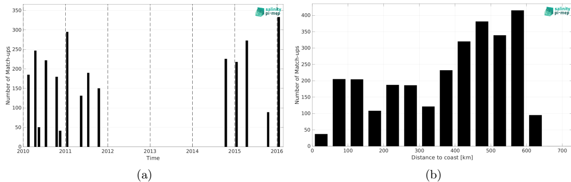
Figure 1: Number of match-ups between TSG (LEGOS-DM) and CCI SSS L4 Merged-OI v3.2 - 7-day running (ESA) SSS as a function of time (a) and as function of the distance to coast (b) over the Bay of Bengal Pi-MEP region and for the full satellite product period.
