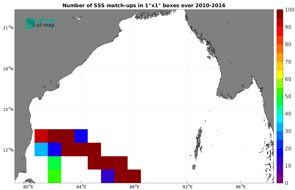
Figure 4: Number of SSS match-ups between TSG (LEGOS-DM) SSS and the CCI SSS L4 Merged-OI v3.2 - 7-day running (ESA) SSS product for the Bay of Bengal Pi-MEP region over 1^\circ \times 1^\circ boxes and for the full satellite product period.
