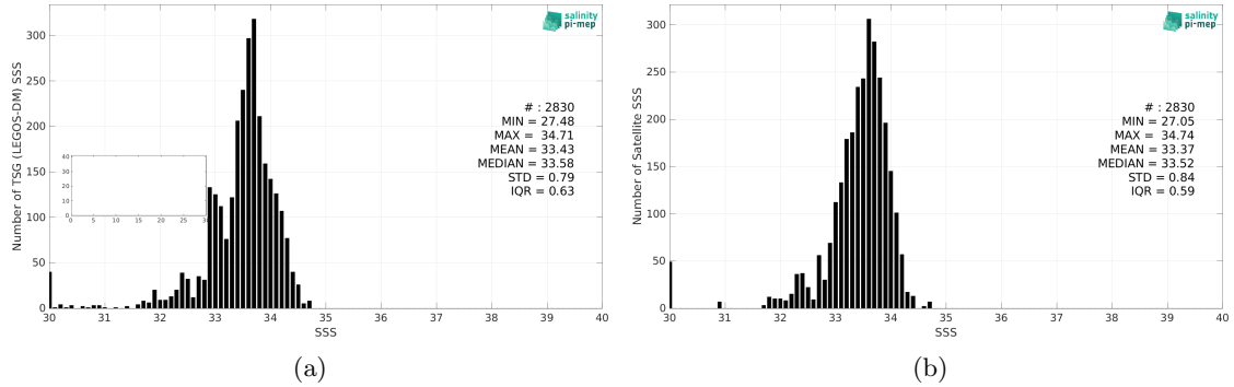
Figure 2: Histograms of SSS from TSG (LEGOS-DM) (a) and CCI SSS L4 Merged-OI v3.2 - 7-day running (ESA) (b) considering all match-up pairs per bins of 0.1 over the Bay of Bengal Pi-MEP region and for the full satellite product period.
