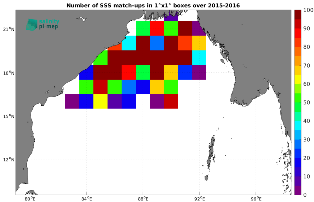
Figure 3: Number of SSS match-ups between Surface drifters SSS and the CCI SSS L4 Merged-OI v3.2 - 7-day running (ESA) SSS product for the Bay of Bengal Pi-MEP region over 1^\circ \times 1^\circ boxes and for the full satellite product period.
