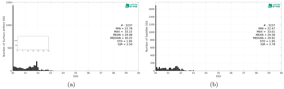
Figure 2: Histograms of SSS from Surface drifters (a) and CCI SSS L4 Merged-OI v3.2 - 7-day running (ESA) (b) considering all match-up pairs per bins of 0.1 over the Bay of Bengal Pi-MEP region and for the full satellite product period.
