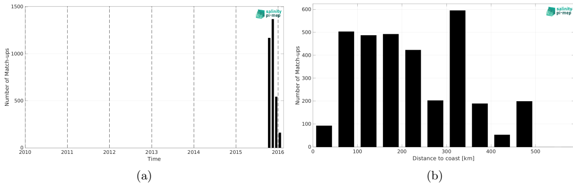
Figure 1: Number of match-ups between Surface drifters and CCI SSS L4 Merged-OI v3.2 - 7-day running (ESA) SSS as a function of time (a) and as function of the distance to coast (b) over the Bay of Bengal Pi-MEP region and for the full satellite product period.
