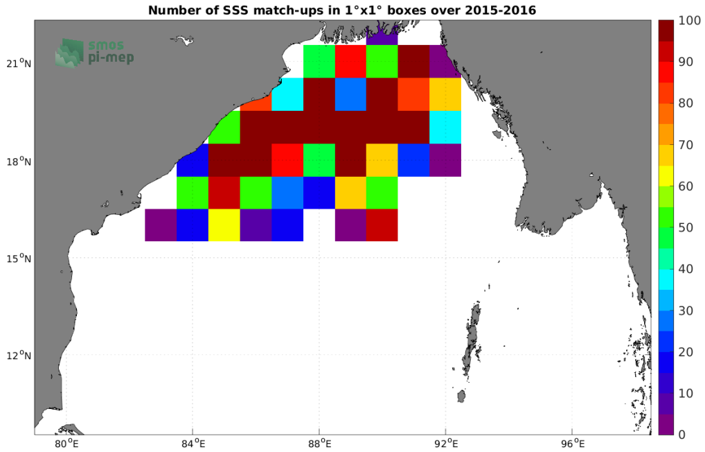
Figure 3: Number of SSS match-ups between Surface drifters SSS and the CCI SSS L4 Merged-OI v3.2 - 7-day running (ESA) SSS product for the Bay of Bengal Pi-MEP region over 1^{\circ} \times 1^{\circ} boxes and for the full satellite product period.
