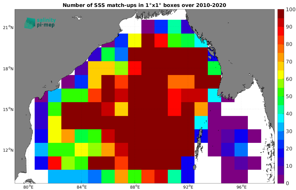
Figure 4: Number of SSS match-ups between Argo SSS and the CCI SSS L4 Merged-OI v3.2 - 7-day running (ESA) SSS product for the Bay of Bengal Pi-MEP region over 1^\circ \times 1^\circ boxes and for the full satellite product period.
