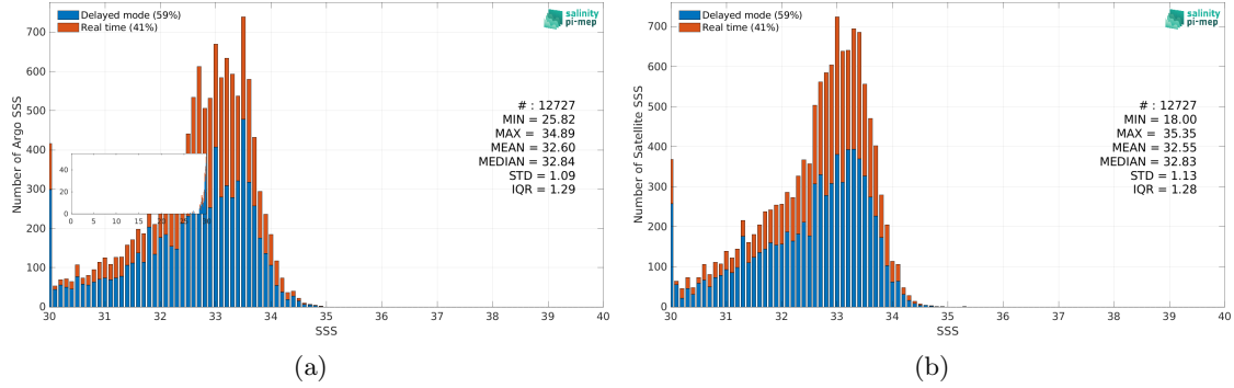
Figure 2: Histograms of SSS from Argo (a) and CCI SSS L4 Merged-OI v3.2 - 7-day running (ESA) (b) considering all match-up pairs per bins of 0.1 over the Bay of Bengal Pi-MEP region and for the full satellite product period.
