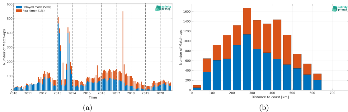
Figure 1: Number of match-ups between Argo and CCI SSS L4 Merged-OI v3.2 - 7-day running (ESA) SSS as a function of time (a) and as function of the distance to coast (b) over the Bay of Bengal Pi-MEP region and for the full satellite product period.
