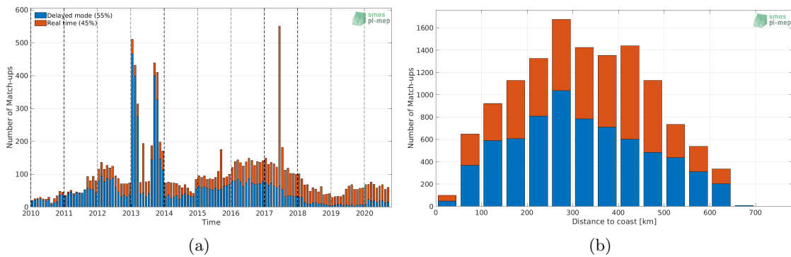
Figure 1: Number of match-ups between Argo and CCI SSS L4 Merged-OI v3.2 - 7-day running (ESA) SSS as a function of time (a) and as function of the distance to coast (b) over the Bay of Bengal Pi-MEP region and for the full satellite product period.
