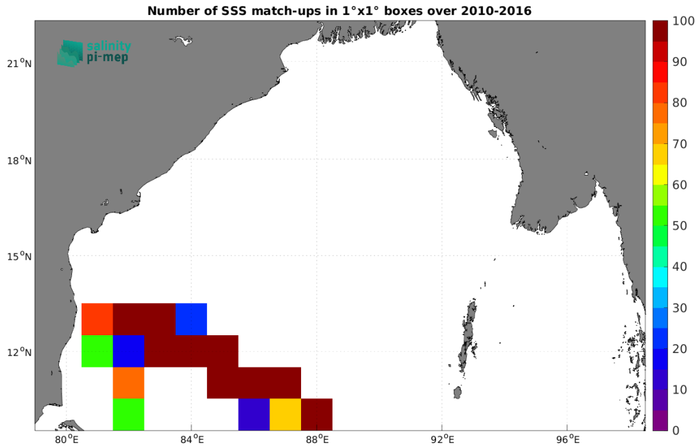
Figure 4: Number of SSS match-ups between TSG (LEGOS-DM) SSS and the CCI SSS L4 Merged-OI v3.2 - 30-day running (ESA) SSS product for the Bay of Bengal Pi-MEP region over 1^\circ \times 1^\circ boxes and for the full satellite product period.
