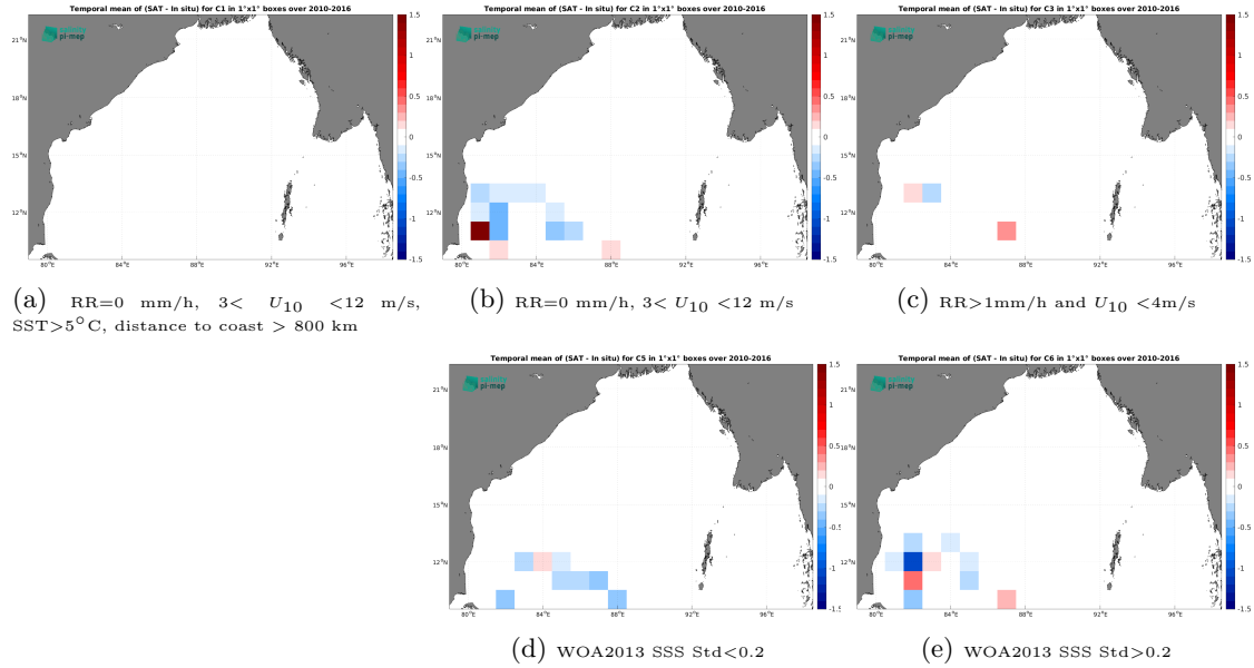
Figure 12: Temporal mean gridded over spatial boxes of size 1^{\circ}\times 1^{\circ} of \Delta\text{SSS} (CCI SSS L4 Merged-OI v3.2 - 30-day running (ESA) - TSG (LEGOS-DM)) for 5 different subdatasets corresponding to:RR=0 mm/h, 3 < U_{10} < 12 m/s, SST > 5^{\circ}\text{C} , distance to coast > 800 km (a), RR=0 mm/h, 3 < U_{10} < 12 m/s (b), RR > 1 mm/h and U_{10} < 4 m/s (c), WOA2013 SSS Std < 0.2 (d), WOA2013 SSS Std > 0.2 (e).
