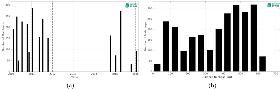
Figure 1: Number of match-ups between TSG (LEGOS-DM) and CCI SSS L4 Merged-OI v3.2 - 30-day running (ESA) SSS as a function of time (a) and as function of the distance to coast (b) over the Bay of Bengal Pi-MEP region and for the full satellite product period.
