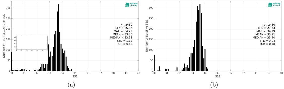
Figure 2: Histograms of SSS from TSG (LEGOS-DM) (a) and CCI SSS L4 Merged-OI v3.2 - 30-day running (ESA) (b) considering all match-up pairs per bins of 0.1 over the Bay of Bengal Pi-MEP region and for the full satellite product period.
