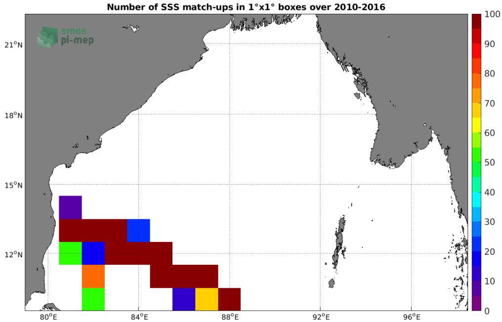
Figure 4: Number of SSS match-ups between TSG (LEGOS-DM) SSS and the CCI SSS L4 Merged-OI v3.2 - 30-day running (ESA) SSS product for the Bay of Bengal Pi-MEP region over 1°x1° boxes and for the full satellite product period.
