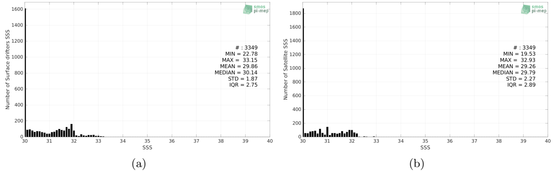
Figure 2: Histograms of SSS from Surface drifters (a) and CCI SSS L4 Merged-OI v3.2 - 30-day running (ESA) (b) considering all match-up pairs per bins of 0.1 over the Bay of Bengal Pi-MEP region and for the full satellite product period.
