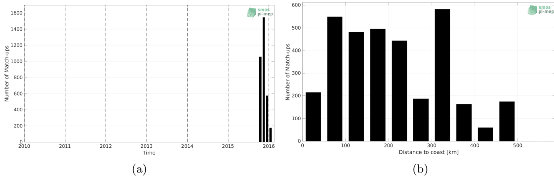
Figure 1: Number of match-ups between Surface drifters and CCI SSS L4 Merged-OI v3.2 - 30-day running (ESA) SSS as a function of time (a) and as function of the distance to coast (b) over the Bay of Bengal Pi-MEP region and for the full satellite product period.
