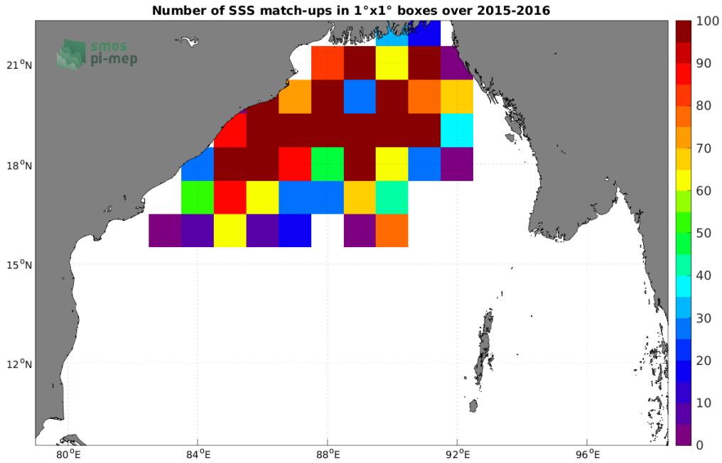
Figure 3: Number of SSS match-ups between Surface drifters SSS and the CCI SSS L4 Merged-OI v3.2 - 30-day running (ESA) SSS product for the Bay of Bengal Pi-MEP region over 1^\circ \times 1^\circ boxes and for the full satellite product period.
