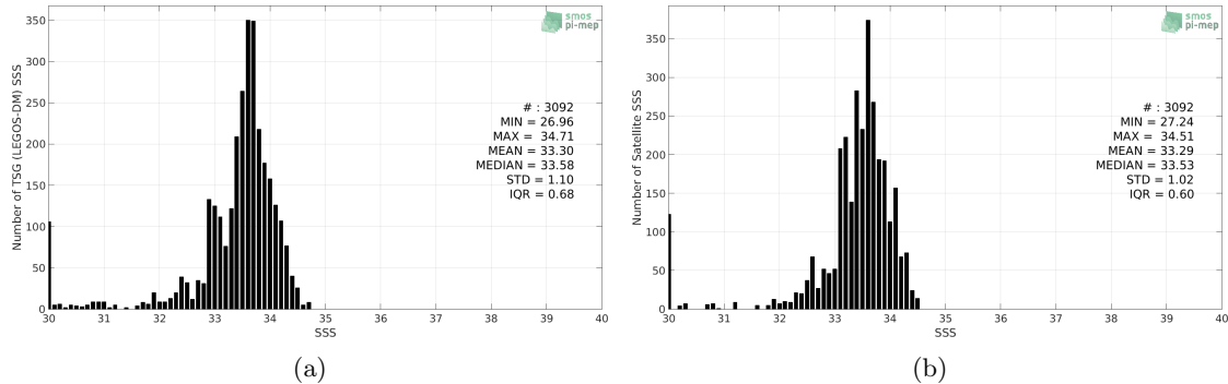
Figure 2: Histograms of SSS from TSG (LEGOS-DM) (a) and CCI SSS L4 Merged-OI v2.31 - 7-day running (ESA) (b) considering all match-up pairs per bins of 0.1 over the Bay of Bengal Pi-MEP region and for the full satellite product period.
