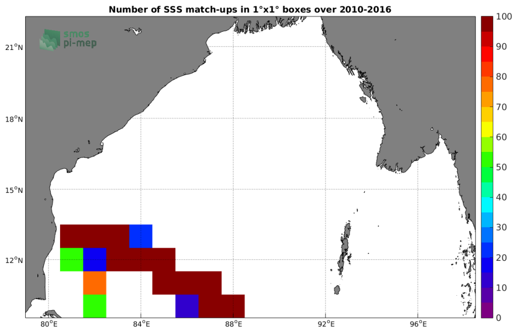
Figure 4: Number of SSS match-ups between TSG (LEGOS-DM) SSS and the CCI SSS L4 Merged-OI v2.31 - 7-day running (ESA) SSS product for the Bay of Bengal Pi-MEP region over 1^\circ \times 1^\circ boxes and for the full satellite product period.
