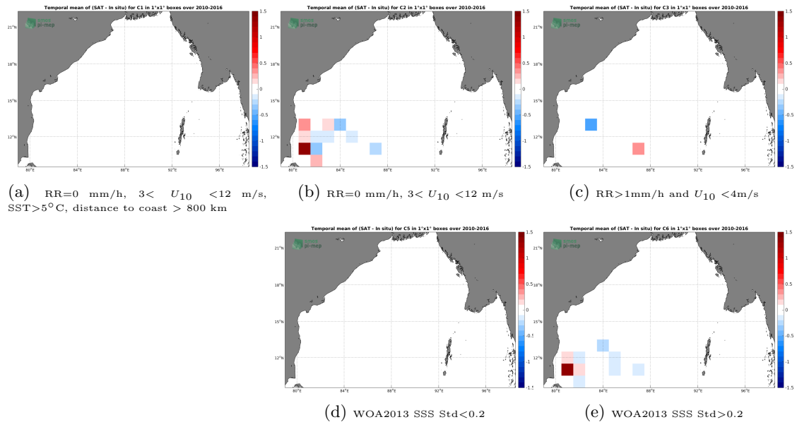
Figure 12: Temporal mean gridded over spatial boxes of size 1^{\circ}\times 1^{\circ} of \Delta\text{SSS} (CCI SSS L4 Merged-OI v2.31 - 7-day running (ESA) - TSG (LEGOS-DM)) for 5 different subdatasets corresponding to:RR=0 mm/h, 3 < U_{10} < 12 m/s, SST >5^{\circ}\text{C} , distance to coast > 800 km (a), RR=0 mm/h, 3 < U_{10} < 12 m/s (b), RR >1 mm/h and U_{10} < 4 m/s (c), WOA2013 SSS Std <0.2 (d), WOA2013 SSS Std >0.2 (e).
