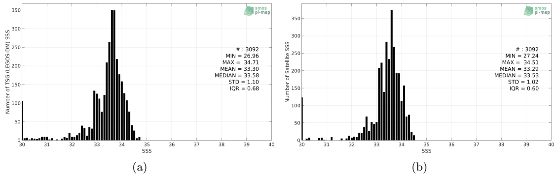
Figure 2: Histograms of SSS from TSG (LEGOS-DM) (a) and CCI L4 Merged-OI v2.31 - 7-day running (ESA) (b) considering all match-up pairs per bins of 0.1 over the Bay of Bengal Pi-MEP region and for the full satellite product period.
