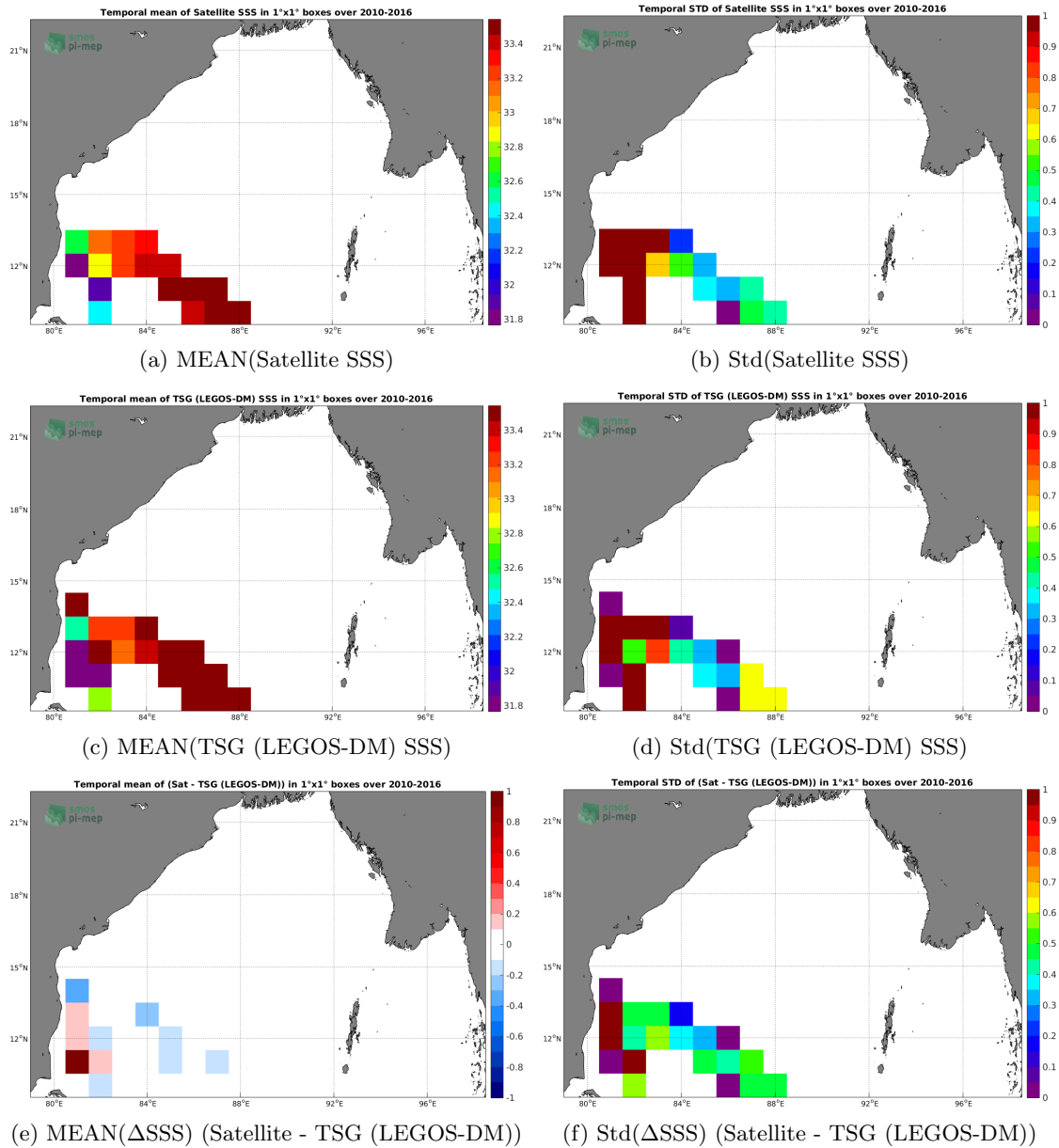
Figure 6: Temporal mean (left) and Std (right) of SSS from CCI L4 Merged-OI v2.31 - 7-day running (ESA) (top), TSG (LEGOS-DM) (middle), and of \Delta SSS (Satellite - TSG (LEGOS-DM)). Only match-up pairs are used to generate these maps.
