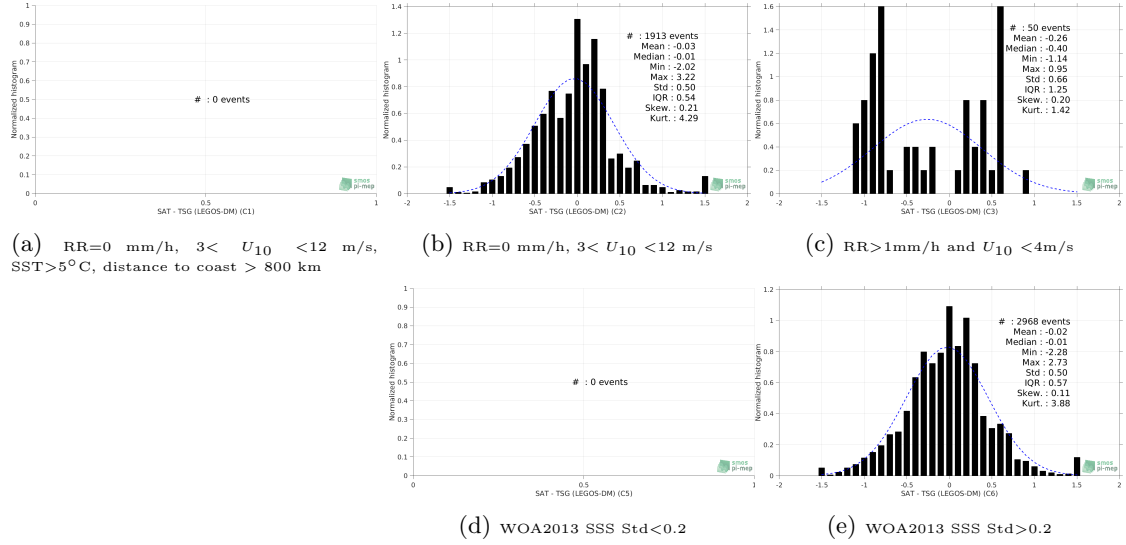
Figure 13: Normalized histogram of \Delta\text{SSS} (CCI L4 Merged-OI v2.31 - 7-day running (ESA) - TSG (LEGOS-DM)) for 5 different subdatasets corresponding to: RR=0 mm/h, 3 < U_{10} < 12 m/s, SST > 5^\circ\text{C} , distance to coast > 800 km (a), RR=0 mm/h, 3 < U_{10} < 12 m/s (b), RR > 1 mm/h and U_{10} < 4 m/s (c), WOA2013 SSS Std < 0.2 (d), WOA2013 SSS Std > 0.2 (e).
