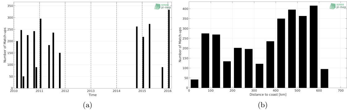
Figure 1: Number of match-ups between TSG (LEGOS-DM) and CCI L4 Merged-OI v2.31 - 7-day running (ESA) SSS as a function of time (a) and as function of the distance to coast (b) over the Bay of Bengal Pi-MEP region and for the full satellite product period.
