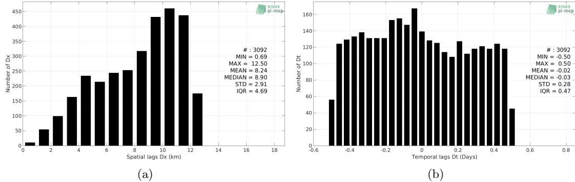
Figure 5: Histograms of the spatial (a) and temporal (b) lags between the time of the TSG (LEGOS-DM) measurements and the date of the corresponding CCI L4 Merged-OI v2.31 - 7-day running (ESA) SSS product.
