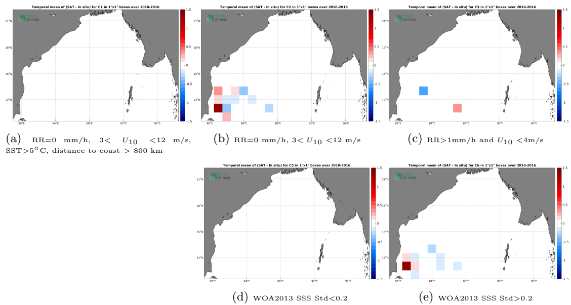
Figure 12: Temporal mean gridded over spatial boxes of size 1°x1° of \Delta SSS (CCI L4 Merged-OI v2.31 - 7-day running (ESA) - TSG (LEGOS-DM)) for 5 different subdatasets corresponding to:RR=0 mm/h, 3 < U_{10} < 12 m/s, SST>5°C, distance to coast > 800 km (a), RR=0 mm/h, 3 < U_{10} < 12 m/s (b), RR>1mm/h and U_{10} < 4 m/s (c), WOA2013 SSS Std<0.2 (d), WOA2013 SSS Std>0.2 (e).
