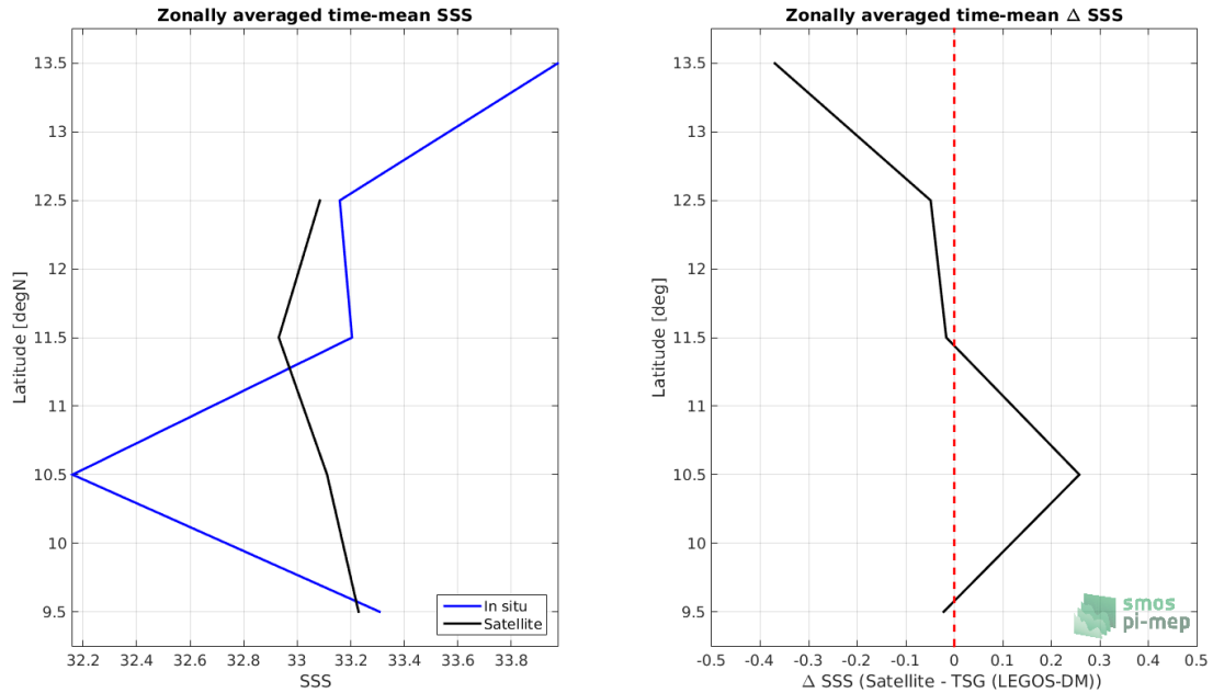
Figure 8: Left panel: Zonal mean SSS from CCI L4 Merged-OI v2.31 - 7-day running (ESA) satellite product (black) and from TSG (LEGOS-DM) (blue). Right panel: Zonal mean of \Delta SSS (Satellite - TSG (LEGOS-DM)) for all the collected Pi-MEP match-up pairs estimated over the full satellite product period.
