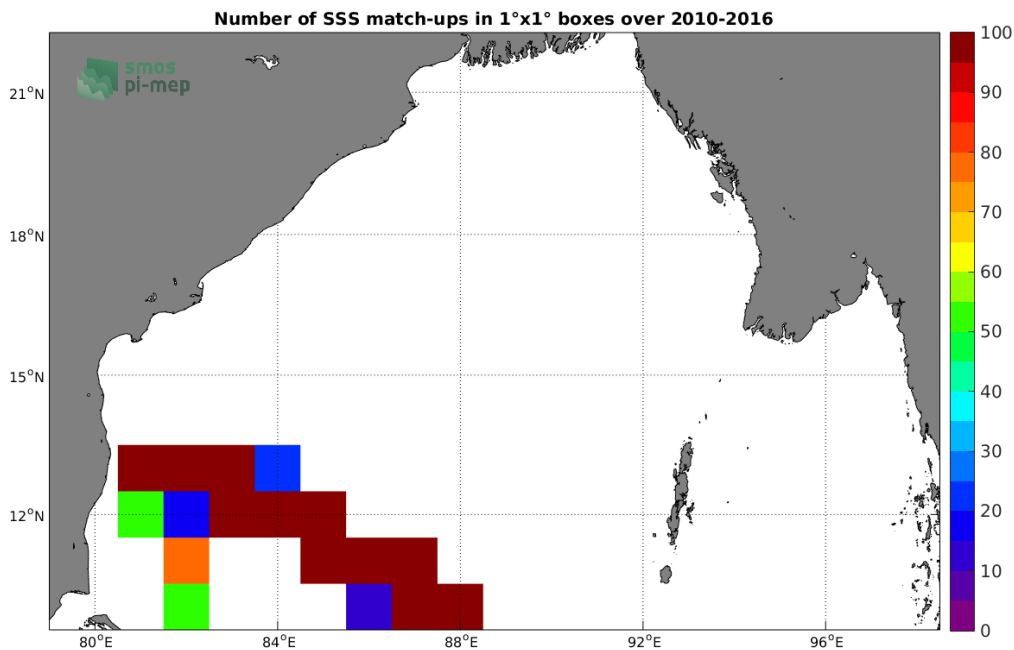
Figure 4: Number of SSS match-ups between TSG (LEGOS-DM) SSS and the CCI L4 Merged-OI v2.31 - 7-day running (ESA) SSS product for the Bay of Bengal Pi-MEP region over 1°x1° boxes and for the full satellite product period.
