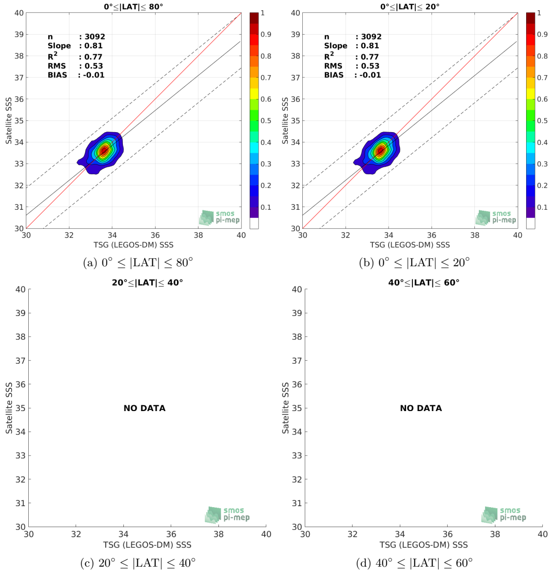
Figure 9: Contour maps of the concentration of CCI L4 Merged-OI v2.31 - 7-day running (ESA) SSS (y-axis) versus TSG (LEGOS-DM) SSS (x-axis) at match-up pairs for different latitude bands. For each plot, the red line shows x=y . The black thin and dashed lines indicate a linear fit through the data cloud and the \pm 95\% confidence levels, respectively. The number match-up pairs n , the slope and R^2 coefficient of the linear fit, the root mean square (RMS) and the mean bias between satellite and in situ data are indicated for each latitude band in each plots.
