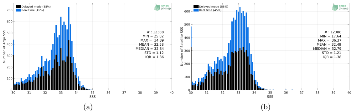
Figure 2: Histograms of SSS from Argo (a) and CCI SSS L4 Merged-OI v2.31 - 7-day running (ESA) (b) considering all match-up pairs per bins of 0.1 over the Bay of Bengal Pi-MEP region and for the full satellite product period.
