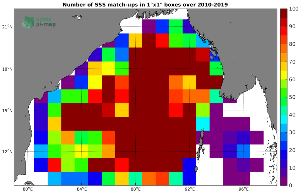
Figure 4: Number of SSS match-ups between Argo SSS and the CCI SSS L4 Merged-OI v2.31 - 7-day running (ESA) SSS product for the Bay of Bengal Pi-MEP region over 1°x1° boxes and for the full satellite product period.
