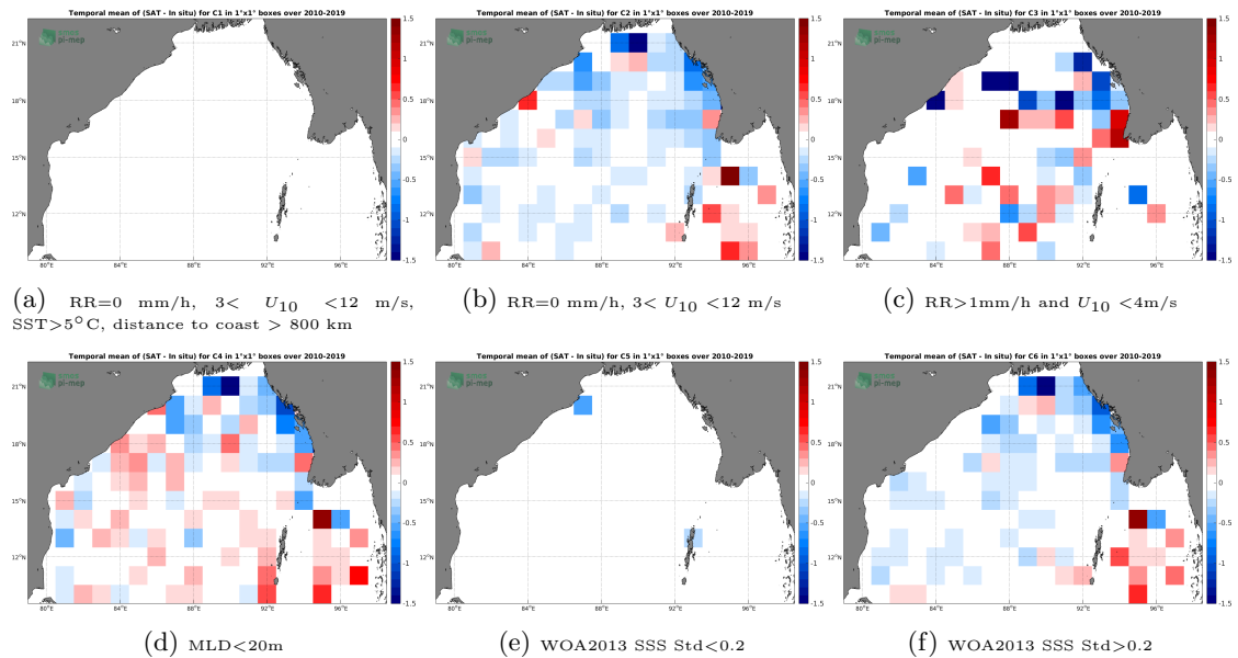
Figure 12: Temporal mean gridded over spatial boxes of size 1^\circ \times 1^\circ of \Delta SSS (CCI SSS L4 Merged-OI v2.31 - 7-day running (ESA) - Argo) for 6 different subdatasets corresponding to:RR=0 mm/h, 3 < U_{10} < 12 m/s, SST > 5^\circ\text{C} , distance to coast > 800 km (a), RR=0 mm/h, 3 < U_{10} < 12 m/s (b), RR > 1 mm/h and U_{10} < 4 m/s (c),MLD < 20 m (d),WOA2013 SSS Std < 0.2 (e),WOA2013 SSS Std > 0.2 (f).
