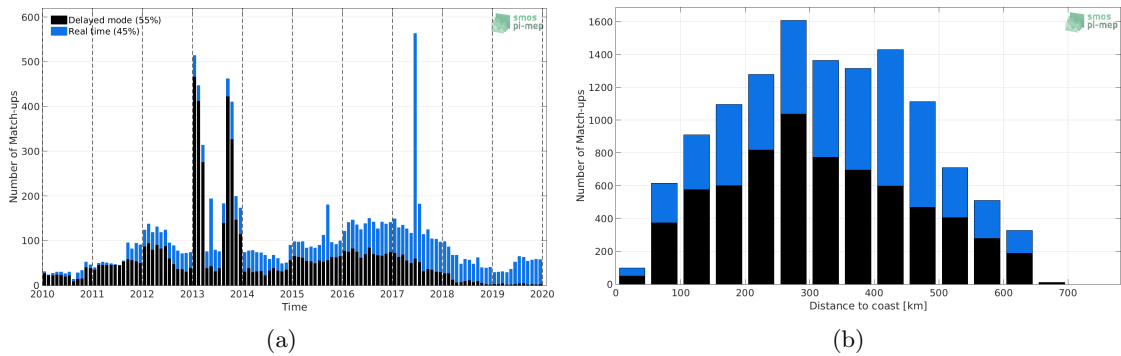
Figure 1: Number of match-ups between Argo and CCI SSS L4 Merged-OI v2.31 - 7-day running (ESA) SSS as a function of time (a) and as function of the distance to coast (b) over the Bay of Bengal Pi-MEP region and for the full satellite product period.
