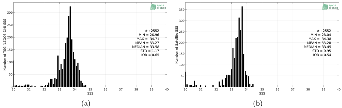
Figure 2: Histograms of SSS from TSG (LEGOS-DM) (a) and CCI SSS L4 Merged-OI v2.31 - 30-day running (ESA) (b) considering all match-up pairs per bins of 0.1 over the Bay of Bengal Pi-MEP region and for the full satellite product period.
