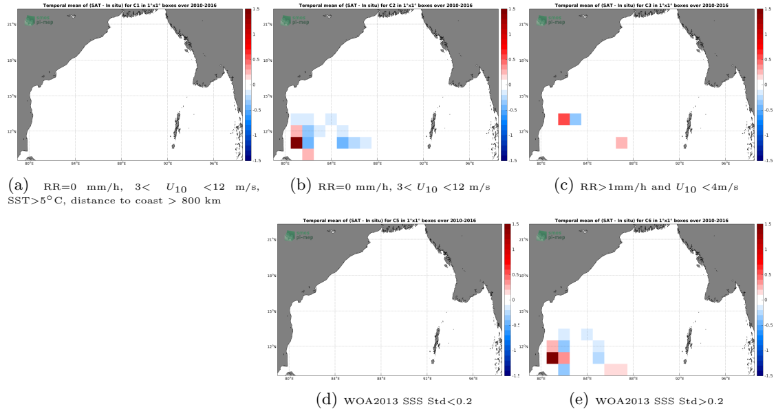
Figure 12: Temporal mean gridded over spatial boxes of size 1^{\circ}\times 1^{\circ} of \Delta\text{SSS} (CCI SSS L4 Merged-OI v2.31 - 30-day running (ESA) - TSG (LEGOS-DM)) for 5 different subdatasets corresponding to:RR=0 mm/h, 3 < U_{10} < 12 m/s, SST >5^{\circ}\text{C} , distance to coast > 800 km (a), RR=0 mm/h, 3 < U_{10} < 12 m/s (b), RR >1 mm/h and U_{10} < 4 m/s (c), WOA2013 SSS Std <0.2 (d), WOA2013 SSS Std >0.2 (e).
