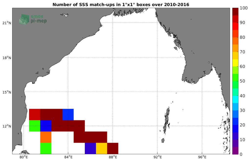
Figure 4: Number of SSS match-ups between TSG (LEGOS-DM) SSS and the CCI SSS L4 Merged-OI v2.31 - 30-day running (ESA) SSS product for the Bay of Bengal Pi-MEP region over 1^\circ \times 1^\circ boxes and for the full satellite product period.
