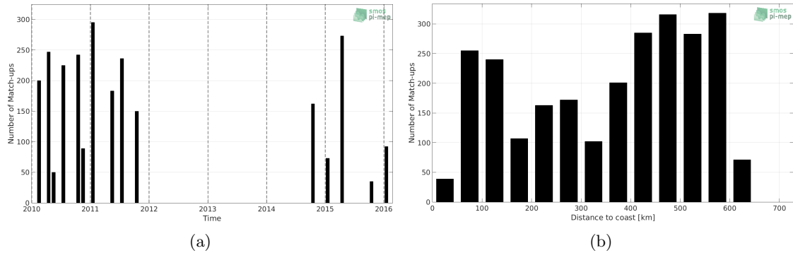
Figure 1: Number of match-ups between TSG (LEGOS-DM) and CCI L4 Merged-OI v2.31 - 30-day running (ESA) SSS as a function of time (a) and as function of the distance to coast (b) over the Bay of Bengal Pi-MEP region and for the full satellite product period.
