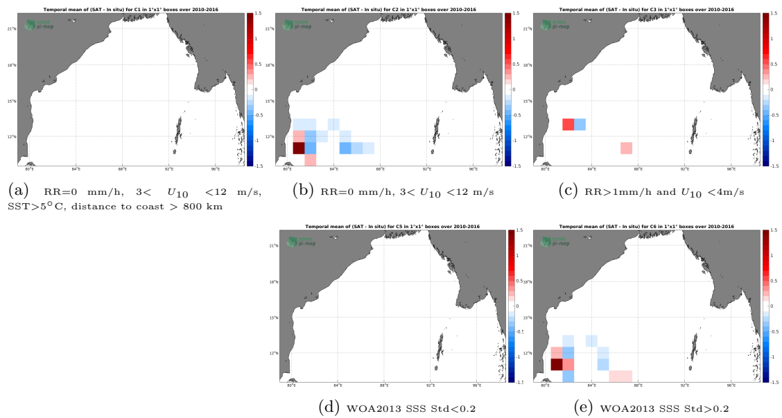
Figure 12: Temporal mean gridded over spatial boxes of size 1°x1° of \Delta SSS (CCI L4 Merged-OI v2.31 - 30-day running (ESA) - TSG (LEGOS-DM)) for 5 different subdatasets corresponding to:RR=0 mm/h, 3 < U_{10} < 12 m/s, SST>5°C, distance to coast > 800 km (a), RR=0 mm/h, 3 < U_{10} < 12 m/s (b), RR>1mm/h and U_{10} < 4 m/s (c), WOA2013 SSS Std<0.2 (d), WOA2013 SSS Std>0.2 (e).
