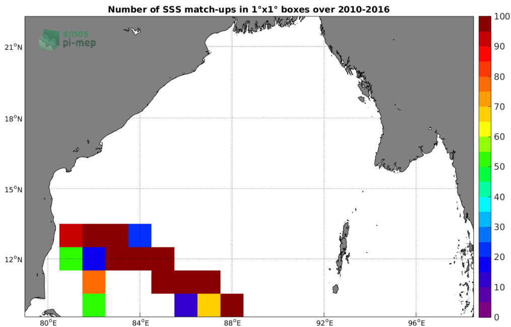
Figure 4: Number of SSS match-ups between TSG (LEGOS-DM) SSS and the CCI L4 Merged-OI v2.31 - 30-day running (ESA) SSS product for the Bay of Bengal Pi-MEP region over 1^\circ \times 1^\circ boxes and for the full satellite product period.
