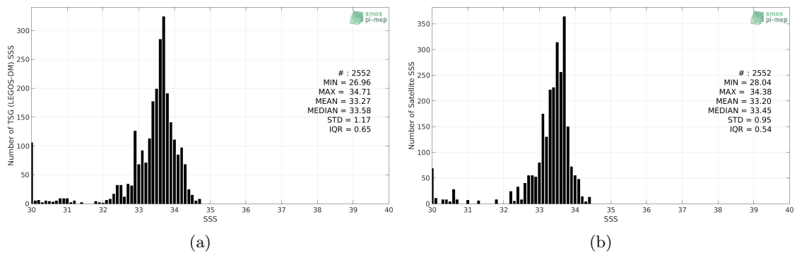
Figure 2: Histograms of SSS from TSG (LEGOS-DM) (a) and CCI L4 Merged-OI v2.31 - 30-day running (ESA) (b) considering all match-up pairs per bins of 0.1 over the Bay of Bengal Pi-MEP region and for the full satellite product period.
