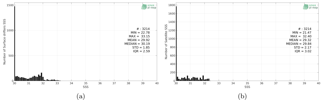
Figure 2: Histograms of SSS from Surface drifters (a) and CCI L4 Merged-OI v2.31 - 30-day running (ESA) (b) considering all match-up pairs per bins of 0.1 over the Bay of Bengal Pi-MEP region and for the full satellite product period.
