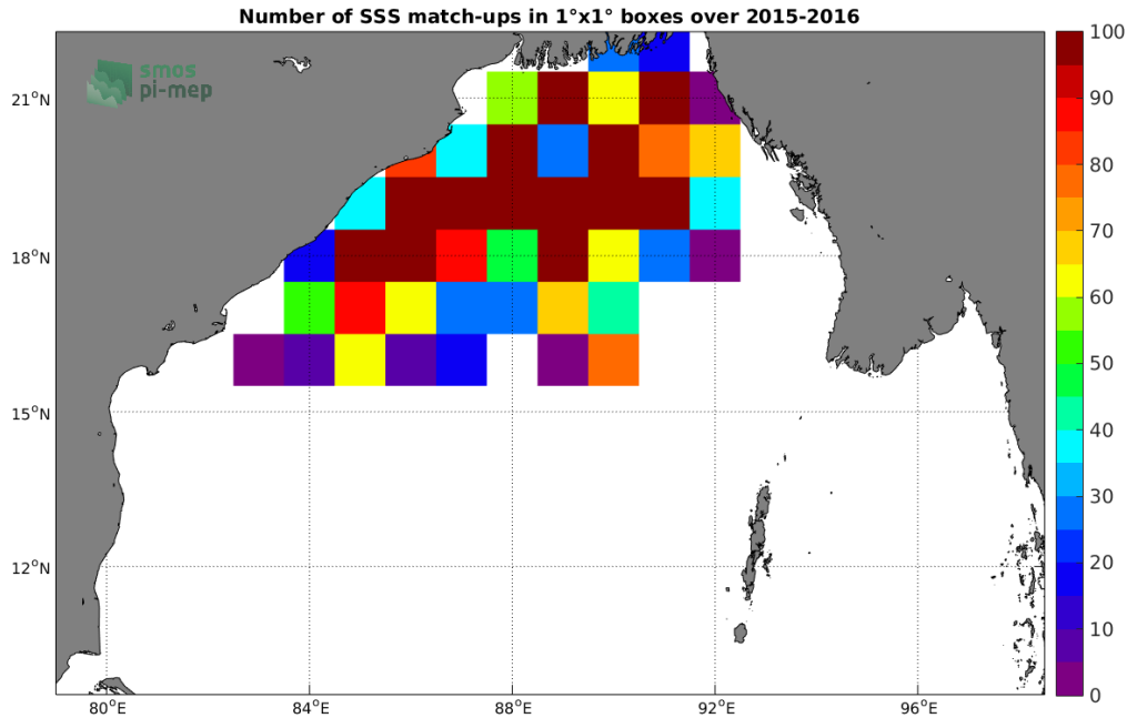
Figure 3: Number of SSS match-ups between Surface drifters SSS and the CCI L4 Merged-OI v2.31 - 30-day running (ESA) SSS product for the Bay of Bengal Pi-MEP region over 1^\circ \times 1^\circ boxes and for the full satellite product period.
