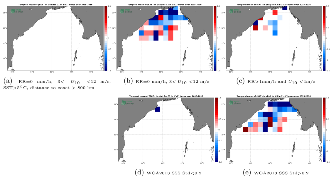
Figure 11: Temporal mean gridded over spatial boxes of size 1°x1° of \Delta SSS (CCI L4 Merged-OI v2.31 - 30-day running (ESA) - Surface drifters) for 5 different subdatasets corresponding to:RR=0 mm/h, 3 < U_{10} < 12 m/s, SST>5°C, distance to coast > 800 km (a), RR=0 mm/h, 3 < U_{10} < 12 m/s (b), RR>1mm/h and U_{10} < 4 m/s (c), WOA2013 SSS Std<0.2 (d), WOA2013 SSS Std>0.2 (e).
