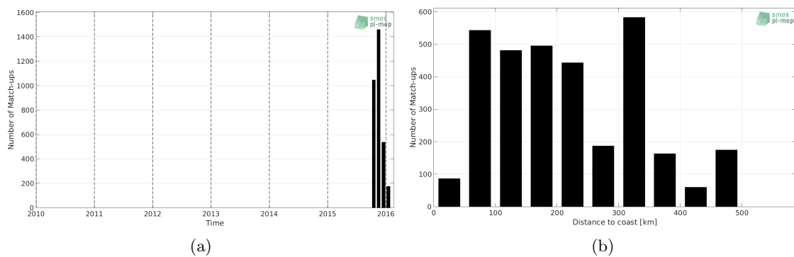
Figure 1: Number of match-ups between Surface drifters and CCI L4 Merged-OI v2.31 - 30-day running (ESA) SSS as a function of time (a) and as function of the distance to coast (b) over the Bay of Bengal Pi-MEP region and for the full satellite product period.
