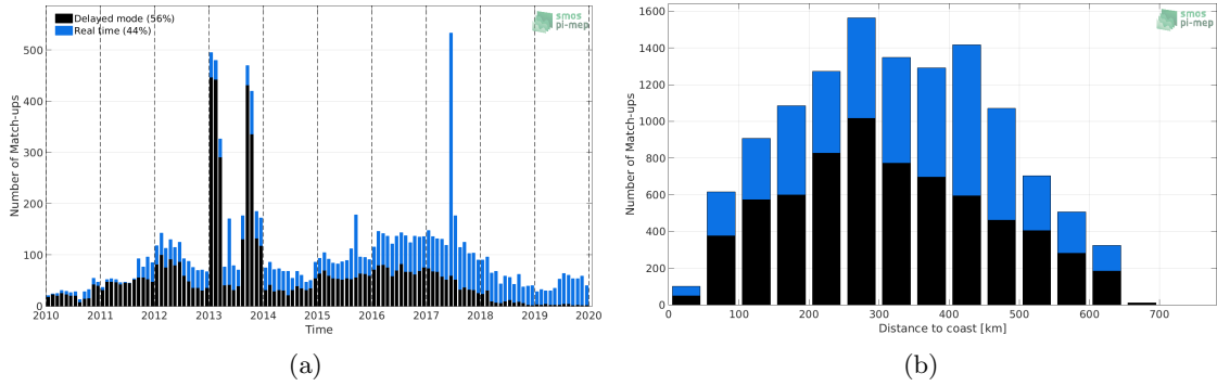
Figure 1: Number of match-ups between Argo and CCI SSS L4 Merged-OI v2.31 - 30-day running (ESA) SSS as a function of time (a) and as function of the distance to coast (b) over the Bay of Bengal Pi-MEP region and for the full satellite product period.
