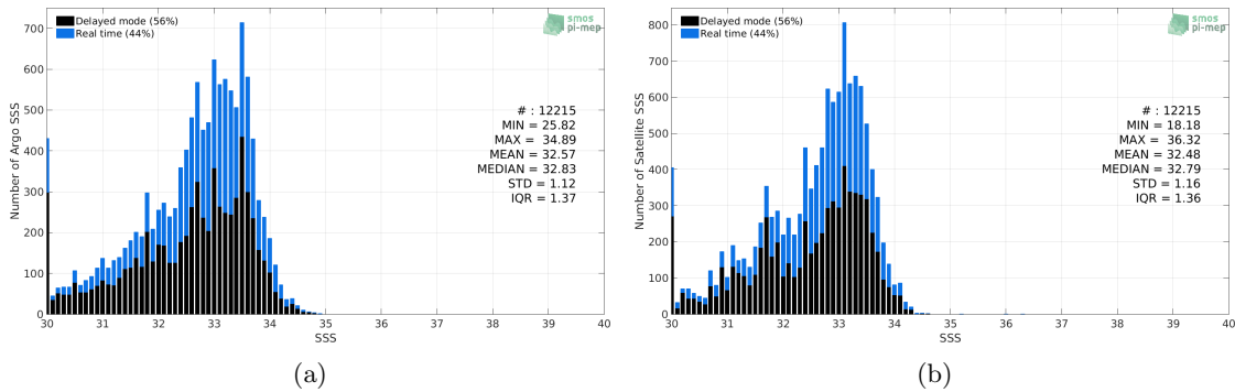
Figure 2: Histograms of SSS from Argo (a) and CCI SSS L4 Merged-OI v2.31 - 30-day running (ESA) (b) considering all match-up pairs per bins of 0.1 over the Bay of Bengal Pi-MEP region and for the full satellite product period.
