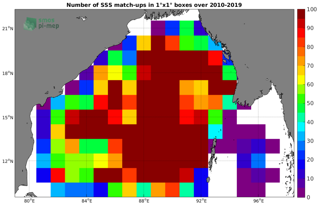
Figure 4: Number of SSS match-ups between Argo SSS and the CCI SSS L4 Merged-OI v2.31 - 30-day running (ESA) SSS product for the Bay of Bengal Pi-MEP region over 1°x1° boxes and for the full satellite product period.
