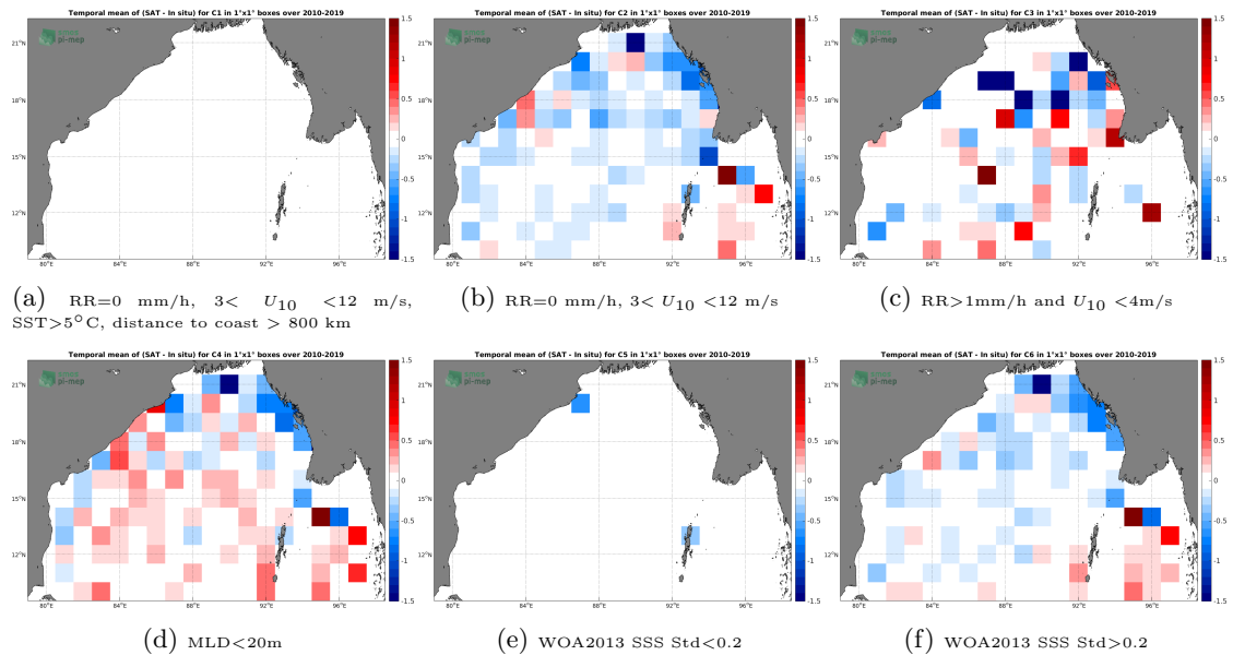
Figure 12: Temporal mean gridded over spatial boxes of size 1^\circ \times 1^\circ of \Delta SSS (CCI SSS L4 Merged-OI v2.31 - 30-day running (ESA) - Argo) for 6 different subdatasets corresponding to:RR=0 mm/h, 3 < U_{10} < 12 m/s, SST > 5^\circ C , distance to coast > 800 km (a), RR=0 mm/h, 3 < U_{10} < 12 m/s (b), RR>1mm/h and U_{10} < 4 m/s (c),MLD<20m (d),WOA2013 SSS Std<0.2 (e),WOA2013 SSS Std>0.2 (f).
