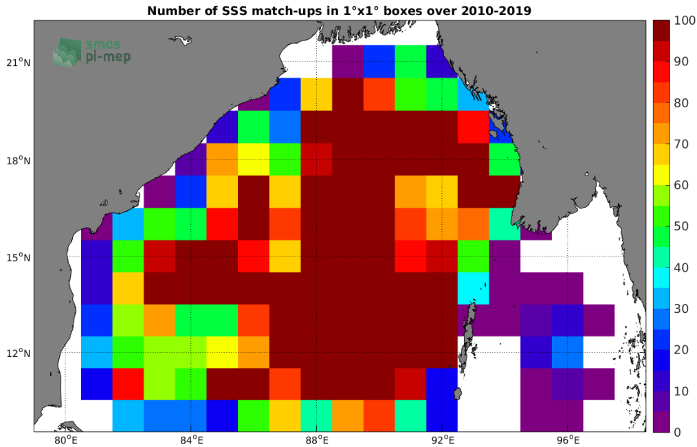
Figure 4: Number of SSS match-ups between Argo SSS and the CCI L4 Merged-OI v2.31 - 30-day running (ESA) SSS product for the Bay of Bengal Pi-MEP region over 1°x1° boxes and for the full satellite product period.
