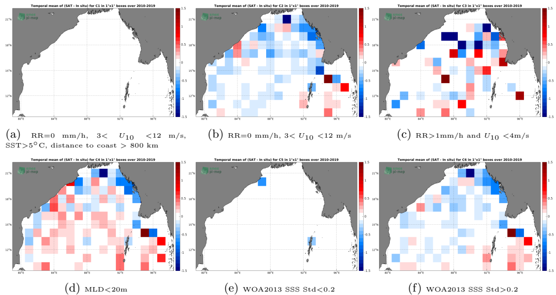
Figure 12: Temporal mean gridded over spatial boxes of size 1^\circ \times 1^\circ of \Delta SSS (CCI L4 Merged-OI v2.31 - 30-day running (ESA) - Argo) for 6 different subdatasets corresponding to:RR=0 mm/h, 3 < U_{10} < 12 m/s, SST >5^\circ C, distance to coast > 800 km (a), RR=0 mm/h, 3 < U_{10} < 12 m/s (b), RR >1 mm/h and U_{10} < 4 m/s (c),MLD <20 m (d),WOA2013 SSS Std <0.2 (e),WOA2013 SSS Std >0.2 (f).
