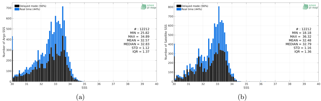
Figure 2: Histograms of SSS from Argo (a) and CCI L4 Merged-OI v2.31 - 30-day running (ESA) (b) considering all match-up pairs per bins of 0.1 over the Bay of Bengal Pi-MEP region and for the full satellite product period.
