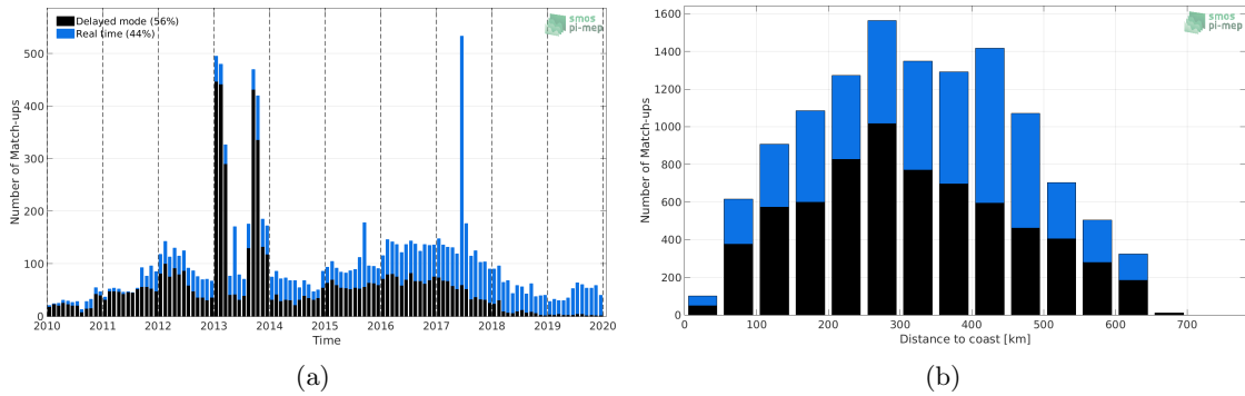
Figure 1: Number of match-ups between Argo and CCI L4 Merged-OI v2.31 - 30-day running (ESA) SSS as a function of time (a) and as function of the distance to coast (b) over the Bay of Bengal Pi-MEP region and for the full satellite product period.
