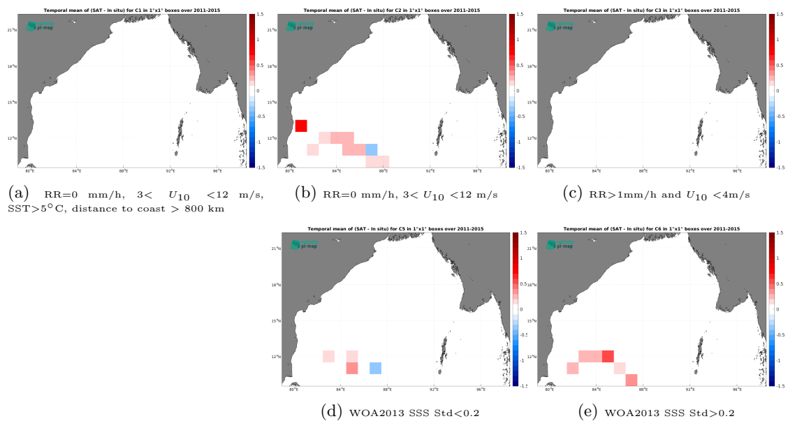
Figure 14: Temporal mean gridded over spatial boxes of size 1^\circ \times 1^\circ of \Delta\text{SSS} (Aquarius SSS L4 OI v5 - Weekly (IPRC) - TSG (LEGOS-DM)) for 5 different subdatasets corresponding to:RR=0 mm/h, 3 < U_{10} < 12 m/s, SST >5^\circ\text{C} , distance to coast > 800 km (a), RR=0 mm/h, 3 < U_{10} < 12 m/s (b), RR >1 mm/h and U_{10} < 4 m/s (c), WOA2013 SSS Std <0.2 (d), WOA2013 SSS Std >0.2 (e).
