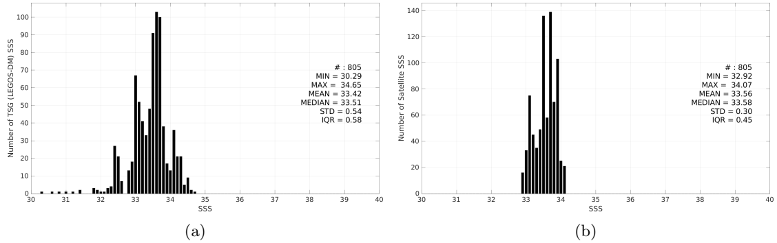
Figure 3: Histograms of SSS from TSG (LEGOS-DM) (a) and Aquarius SSS L4 OI v5 - Weekly (IPRC) (b) considering all match-up pairs per bins of 0.1 over the Bay of Bengal Pi-MEP region and for the full satellite product period.
