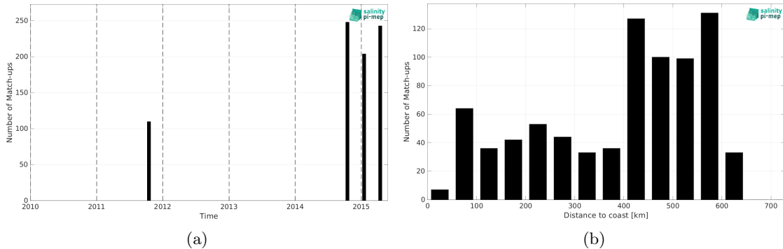
Figure 2: Number of match-ups between TSG (LEGOS-DM) and Aquarius SSS L4 OI v5 - Weekly (IPRC) SSS as a function of time (a) and as function of the distance to coast (b) over the Bay of Bengal Pi-MEP region and for the full satellite product period.
