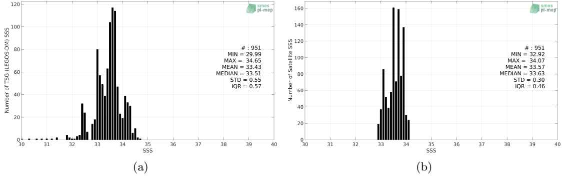
Figure 2: Histograms of SSS from TSG (LEGOS-DM) (a) and Aquarius SSS L4 OI v5 - Weekly (IPRC) (b) considering all match-up pairs per bins of 0.1 over the Bay of Bengal Pi-MEP region and for the full satellite product period.
