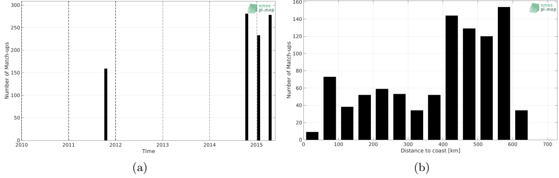
Figure 1: Number of match-ups between TSG (LEGOS-DM) and Aquarius SSS L4 OI v5 - Weekly (IPRC) SSS as a function of time (a) and as function of the distance to coast (b) over the Bay of Bengal Pi-MEP region and for the full satellite product period.
