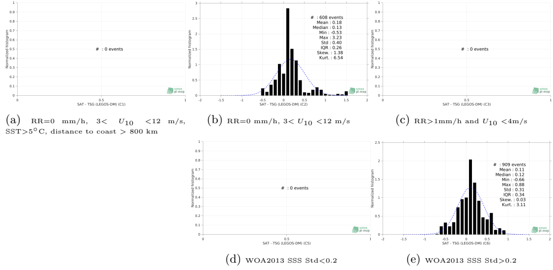
Figure 13: Normalized histogram of \Delta\text{SSS} (Aquarius SSS L4 OI v5 - Weekly (IPRC) - TSG (LEGOS-DM)) for 5 different subdatasets corresponding to: RR=0 mm/h, 3 < U_{10} < 12 m/s, SST > 5^\circ\text{C} , distance to coast > 800 km (a), RR=0 mm/h, 3 < U_{10} < 12 m/s (b), RR > 1\text{mm/h} and U_{10} < 4\text{m/s} (c), WOA2013 SSS Std < 0.2 (d), WOA2013 SSS Std > 0.2 (e).
