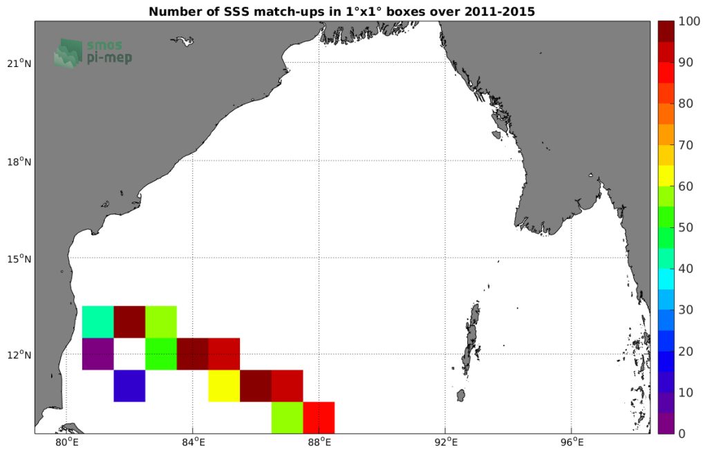
Figure 4: Number of SSS match-ups between TSG-LEGOS-DM SSS and the Aquarius-L4-IPRC-V5-WEEKLY SSS product for the Bay of Bengal Pi-MEP region over 1°x1° boxes and for the full satellite product period.
