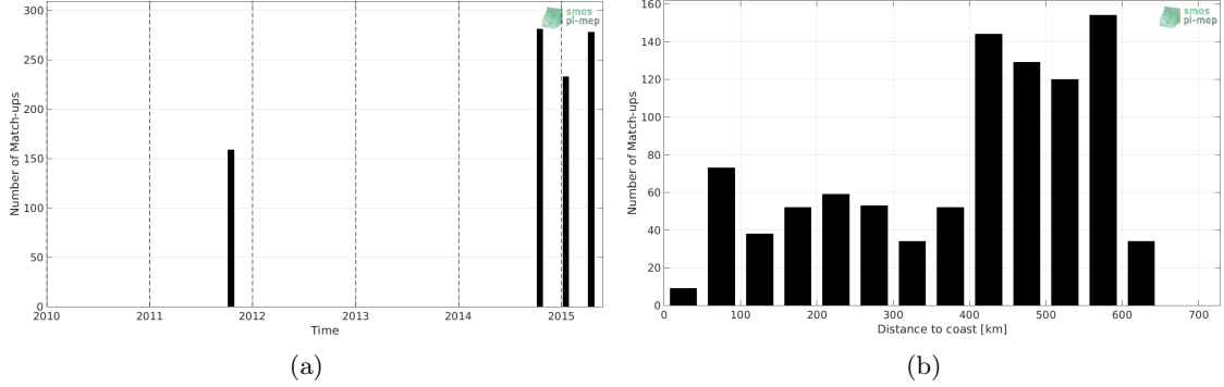
Figure 1: Number of match-ups between TSG-LEGOS-DM and Aquarius-L4-IPRC-V5-WEEKLY SSS as a function of time (a) and as function of the distance to coast (b) over the Bay of Bengal Pi-MEP region and for the full satellite product period.
