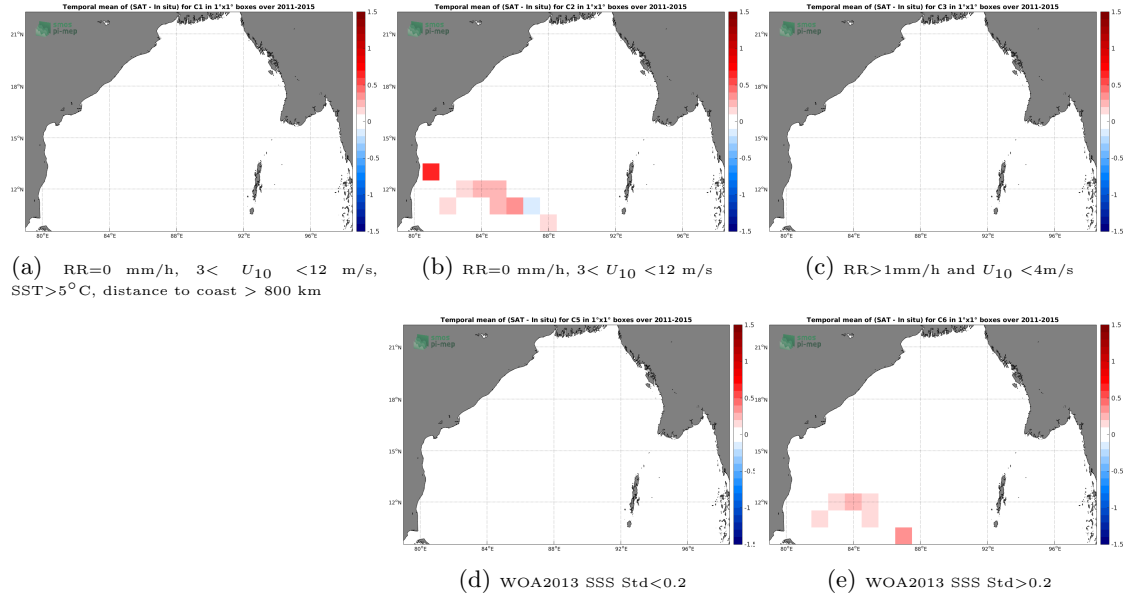
Figure 12: Temporal mean gridded over spatial boxes of size 1^\circ \times 1^\circ of \Delta SSS (Aquarius-L4-IPRC-V5-WEEKLY - TSG-LEGOS-DM) for 5 different subdatasets corresponding to: RR=0 mm/h, 3 < U_{10} < 12 m/s, SST > 5^\circ\text{C} , distance to coast > 800 km (a), RR=0 mm/h, 3 < U_{10} < 12 m/s (b), RR > 1\text{mm/h} and U_{10} < 4\text{m/s} (c), WOA2013 SSS Std < 0.2 (d), WOA2013 SSS Std > 0.2 (e).
