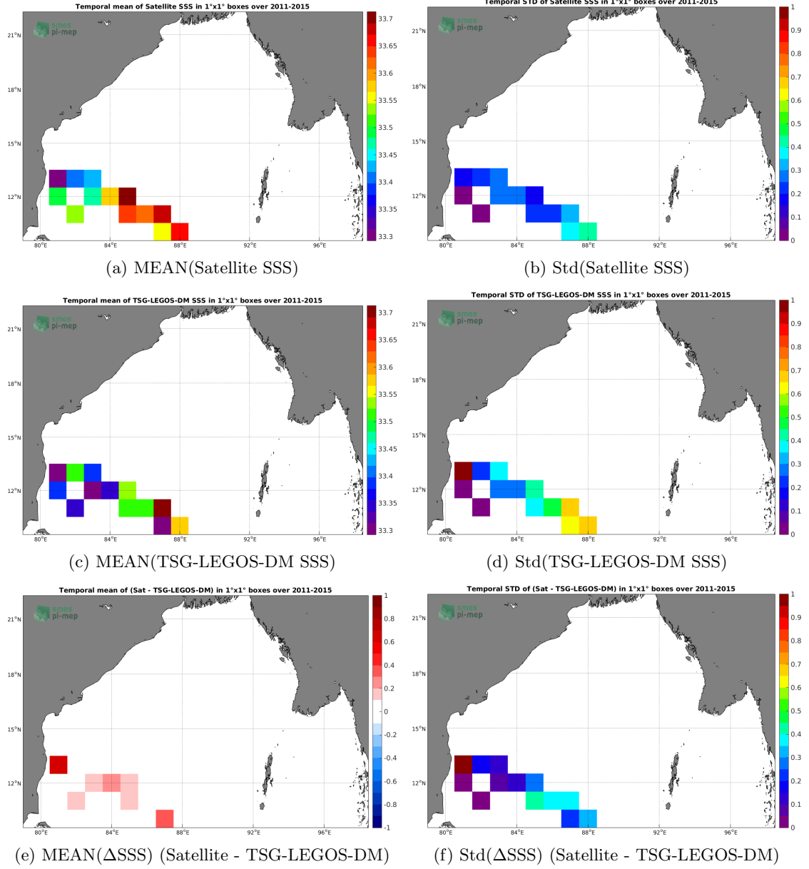
Figure 6: Temporal mean (left) and Std (right) of SSS from Aquarius-L4-IPRC-V5-WEEKLY (top), TSG-LEGOS-DM (middle), and of \Delta SSS (Satellite - TSG-LEGOS-DM). Only match-up pairs are used to generate these maps.
