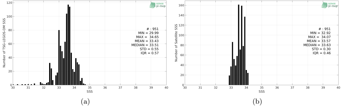
Figure 2: Histograms of SSS from TSG-LEGOS-DM (a) and Aquarius-L4-IPRC-V5-WEEKLY (b) considering all match-up pairs per bins of 0.1 over the Bay of Bengal Pi-MEP region and for the full satellite product period.
