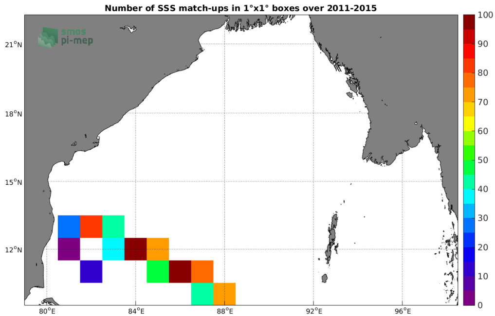
Figure 4: Number of SSS match-ups between TSG-LEGOS-DM SSS and the Aquarius-L4-IPRC-V5-WEEKLY SSS product for the Bay of Bengal Pi-MEP region over 1^\circ \times 1^\circ boxes and for the full satellite product period.
