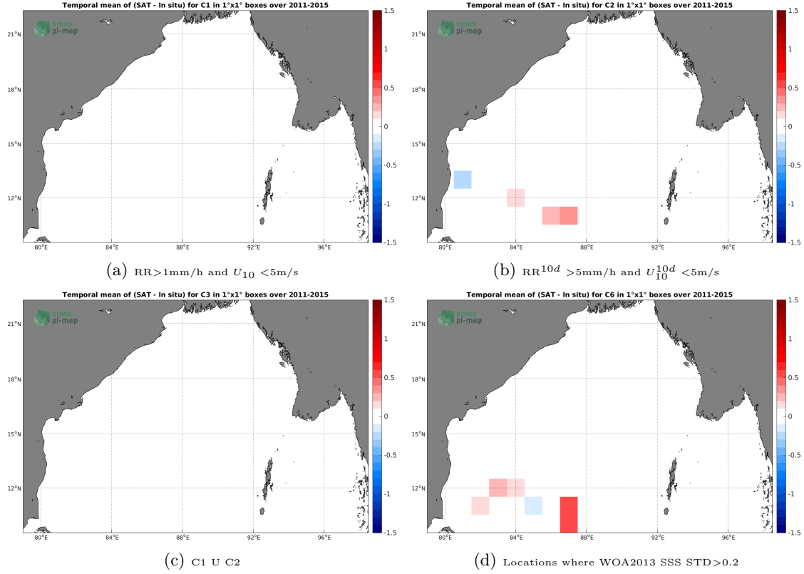
Figure 12: Temporal mean gridded over spatial boxes of size 1^\circ \times 1^\circ of \Delta SSS (Aquarius-L4-IPRC-V5-WEEKLY - TSG-LEGOS-DM) for 4 different subdatasets corresponding to: RR > 1\text{mm/h} and U_{10} < 5\text{m/s} (a), RR^{10d} > 5\text{mm/h} and U_{10}^{10d} < 5\text{m/s} (b), C1 U C2 (c), Locations where WOA2013 SSS STD > 0.2 (d).
