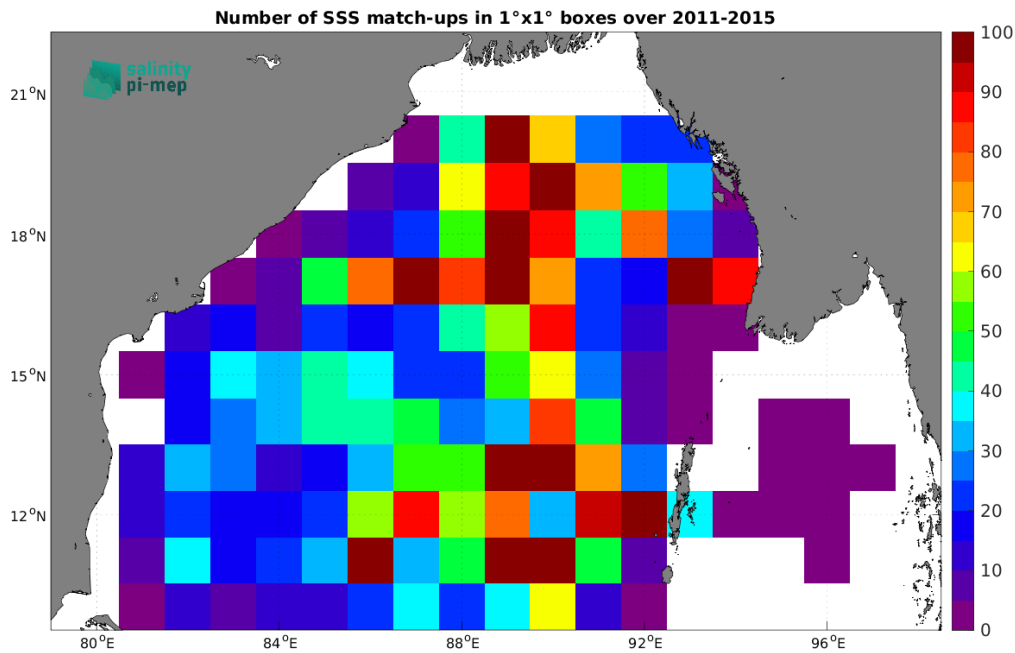
Figure 5: Number of SSS match-ups between Argo SSS and the Aquarius SSS L4 OI v5 - Weekly (IPRC) SSS product for the Bay of Bengal Pi-MEP region over 1^\circ \times 1^\circ boxes and for the full satellite product period.
