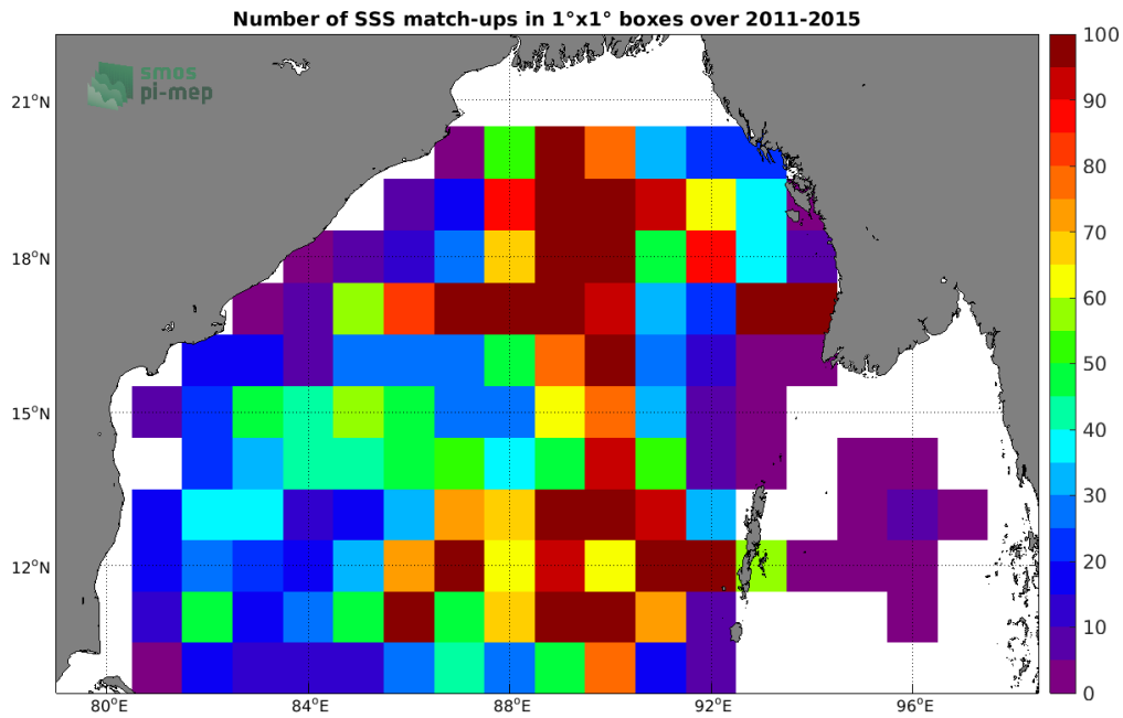
Figure 4: Number of SSS match-ups between Argo SSS and the Aquarius SSS L4 OI v5 - Weekly (IPRC) SSS product for the Bay of Bengal Pi-MEP region over 1^\circ \times 1^\circ boxes and for the full satellite product period.
