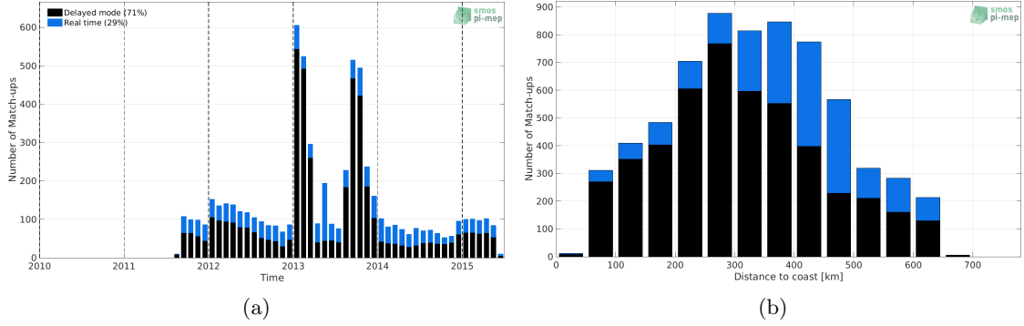
Figure 1: Number of match-ups between Argo and Aquarius SSS L4 OI v5 - Weekly (IPRC) SSS as a function of time (a) and as function of the distance to coast (b) over the Bay of Bengal Pi-MEP region and for the full satellite product period.
