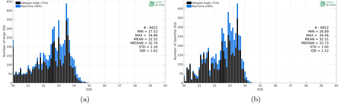
Figure 2: Histograms of SSS from Argo (a) and Aquarius SSS L4 OI v5 - Weekly (IPRC) (b) considering all match-up pairs per bins of 0.1 over the Bay of Bengal Pi-MEP region and for the full satellite product period.
