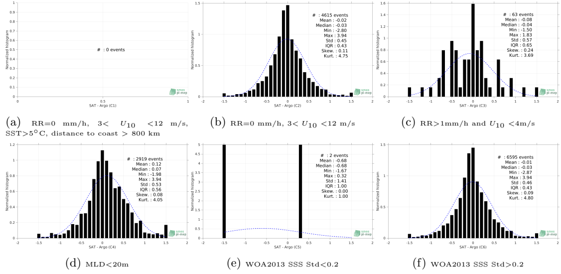
Figure 13: Normalized histogram of \Delta SSS (Aquarius SSS L4 OI v5 - Weekly (IPRC) - Argo) for 6 different subdatasets corresponding to: RR=0 mm/h, 3 < U_{10} < 12 m/s, SST > 5^\circ C , distance to coast > 800 km (a), RR=0 mm/h, 3 < U_{10} < 12 m/s (b), RR > 1 mm/h and U_{10} < 4 m/s (c), MLD < 20 m (d), WOA2013 SSS Std < 0.2 (e), WOA2013 SSS Std > 0.2 (f).
